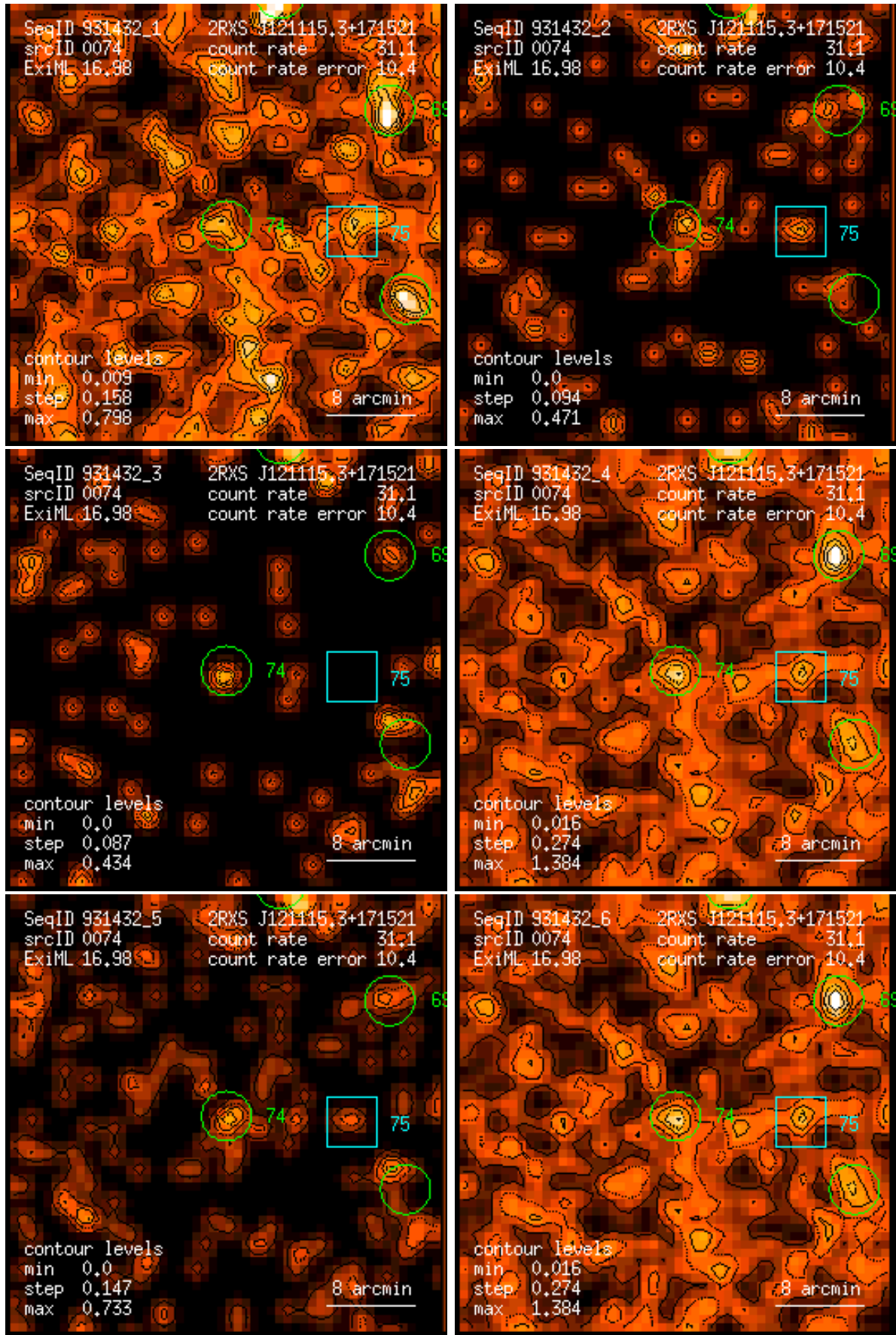
Figure 74: RASS 931432: detection 0074: band rate images, Gaussian filter: (1) PSPC channels 11 – 41, (2) 52 – 90, (3) 91 – 201, (4) 11 – 235, (5) 52 – 201, (6) 11 – 201. Broad band rates in counts/ks. Band rate contour levels in counts/ks/arcmin 2 .
