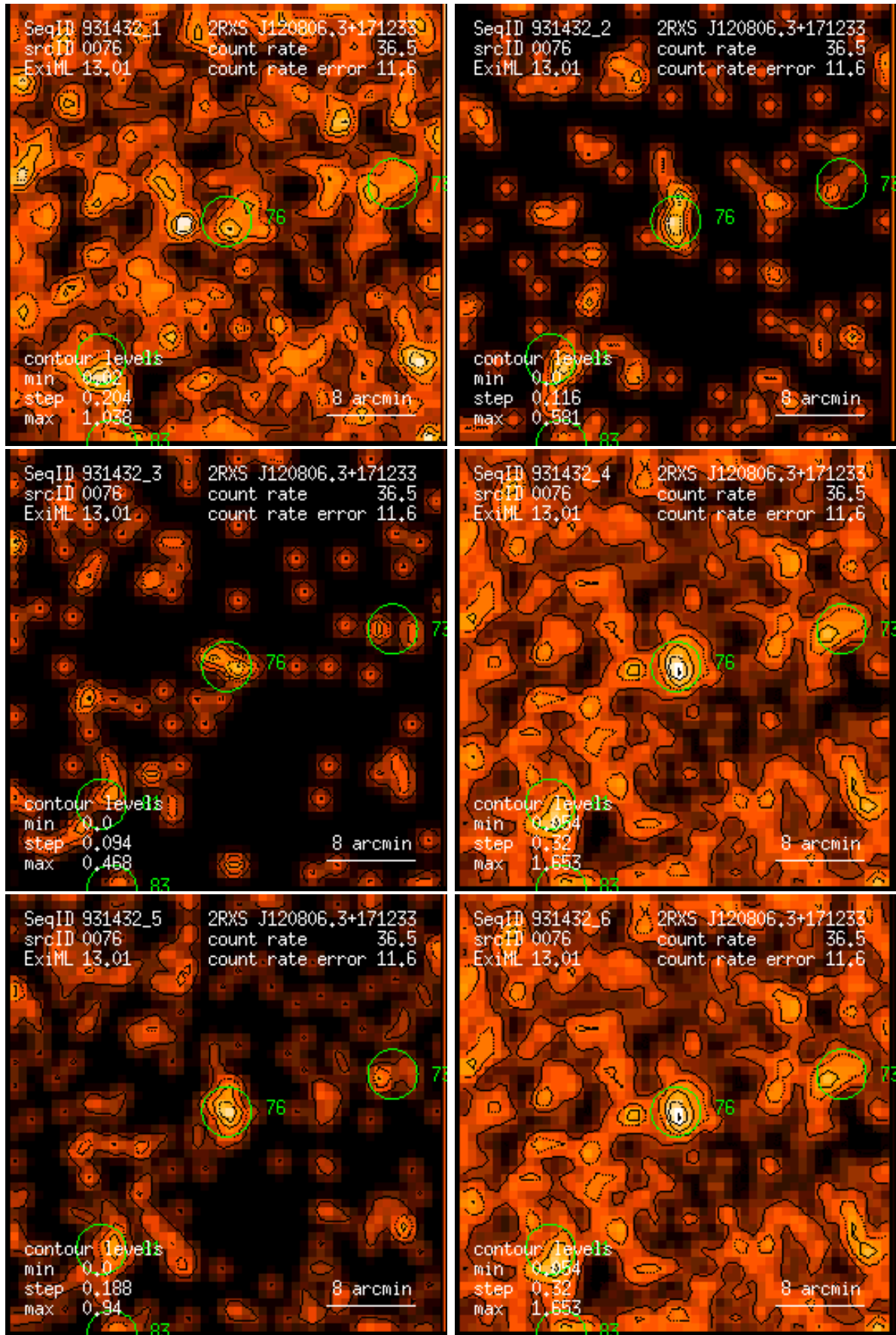
Figure 76: RASS 931432: detection 0076: band rate images, Gaussian filter: (1) PSPC channels 11 – 41, (2) 52 – 90, (3) 91 – 201, (4) 11 – 235, (5) 52 – 201, (6) 11 – 201. Broad band rates in counts/ks. Band rate contour levels in counts/ks/arcmin 2 .
