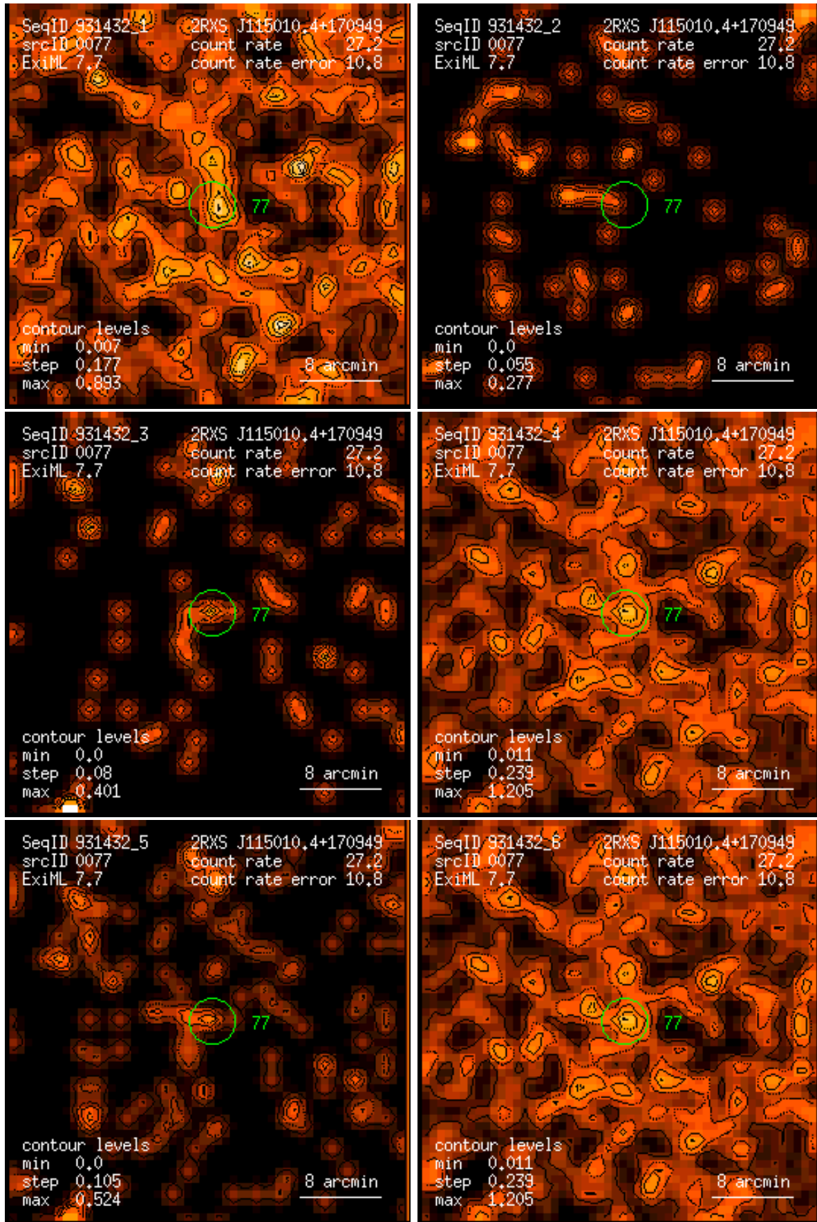
Figure 77: RASS 931432: detection 0077: band rate images, Gaussian filter: (1) PSPC channels 11 – 41, (2) 52 – 90, (3) 91 – 201, (4) 11 – 235, (5) 52 – 201, (6) 11 – 201. Broad band rates in counts/ks. Band rate contour levels in counts/ks/arcmin 2 .
