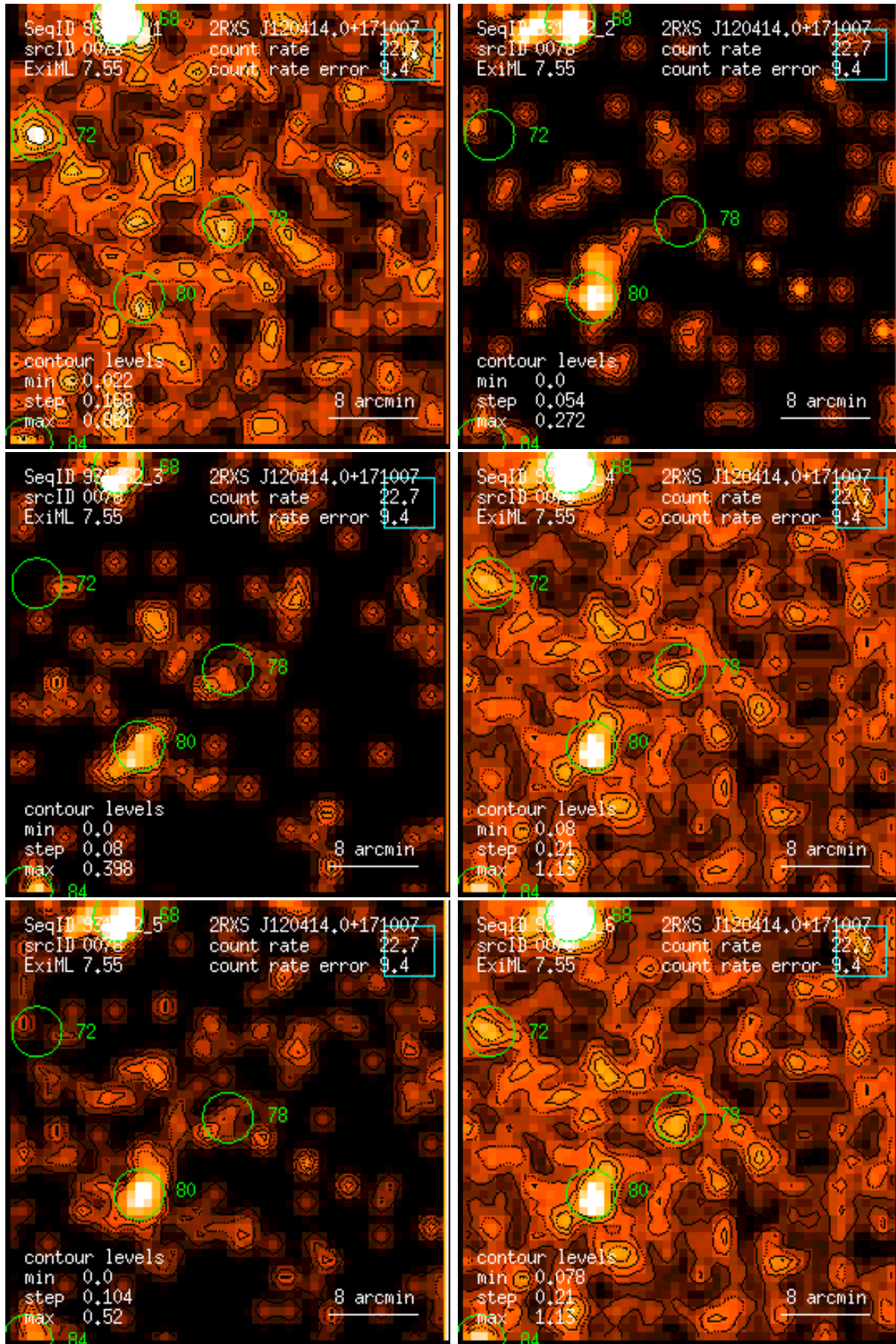
Figure 78: RASS 931432: detection 0078: band rate images, Gaussian filter: (1) PSPC channels 11 – 41, (2) 52 – 90, (3) 91 – 201, (4) 11 – 235, (5) 52 – 201, (6) 11 – 201. Broad band rates in counts/ks. Band rate contour levels in counts/ks/arcmin 2 .
