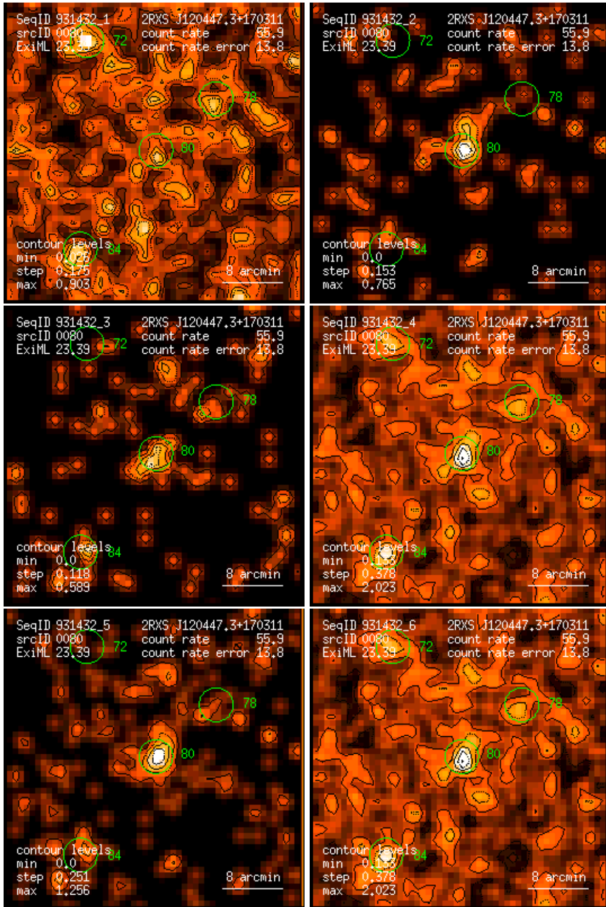
Figure 80: RASS 931432: detection 0080: band rate images, Gaussian filter: (1) PSPC channels 11 – 41, (2) 52 – 90, (3) 91 – 201, (4) 11 – 235, (5) 52 – 201, (6) 11 – 201. Broad band rates in counts/ks. Band rate contour levels in counts/ks/arcmin 2 .
