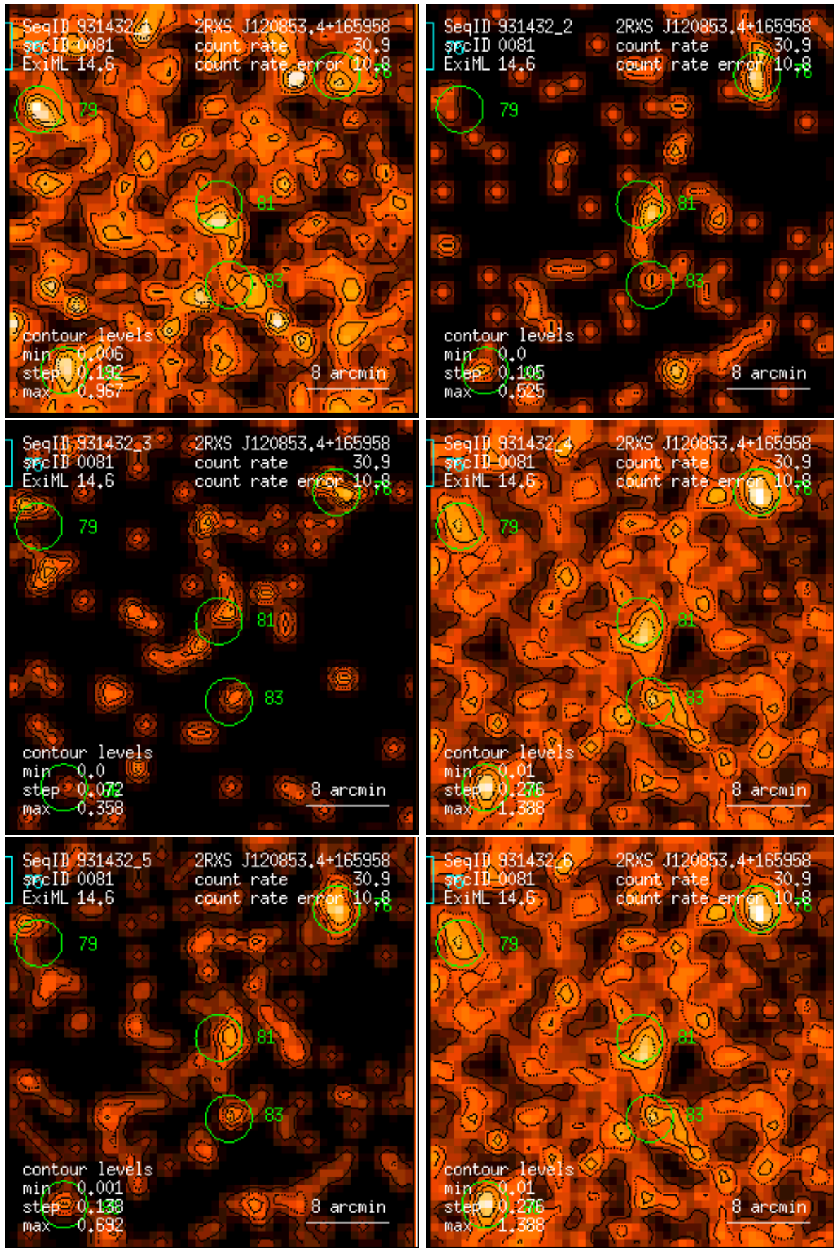
Figure 81: RASS 931432: detection 0081: band rate images, Gaussian filter: (1) PSPC channels 11 – 41, (2) 52 – 90, (3) 91 – 201, (4) 11 – 235, (5) 52 – 201, (6) 11 – 201. Broad band rates in counts/ks. Band rate contour levels in counts/ks/arcmin 2 .
