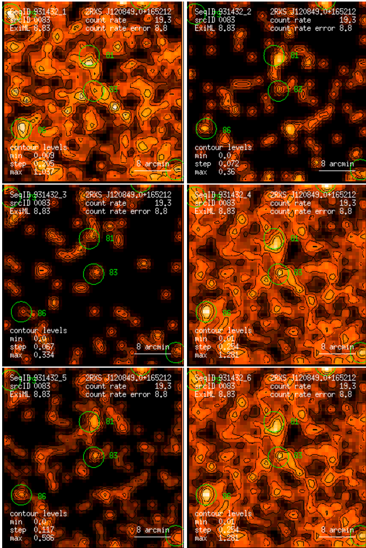
Figure 83: RASS 931432: detection 0083: band rate images, Gaussian filter: (1) PSPC channels 11 – 41, (2) 52 – 90, (3) 91 – 201, (4) 11 – 235, (5) 52 – 201, (6) 11 – 201. Broad band rates in counts/ks. Band rate contour levels in counts/ks/arcmin 2 .
