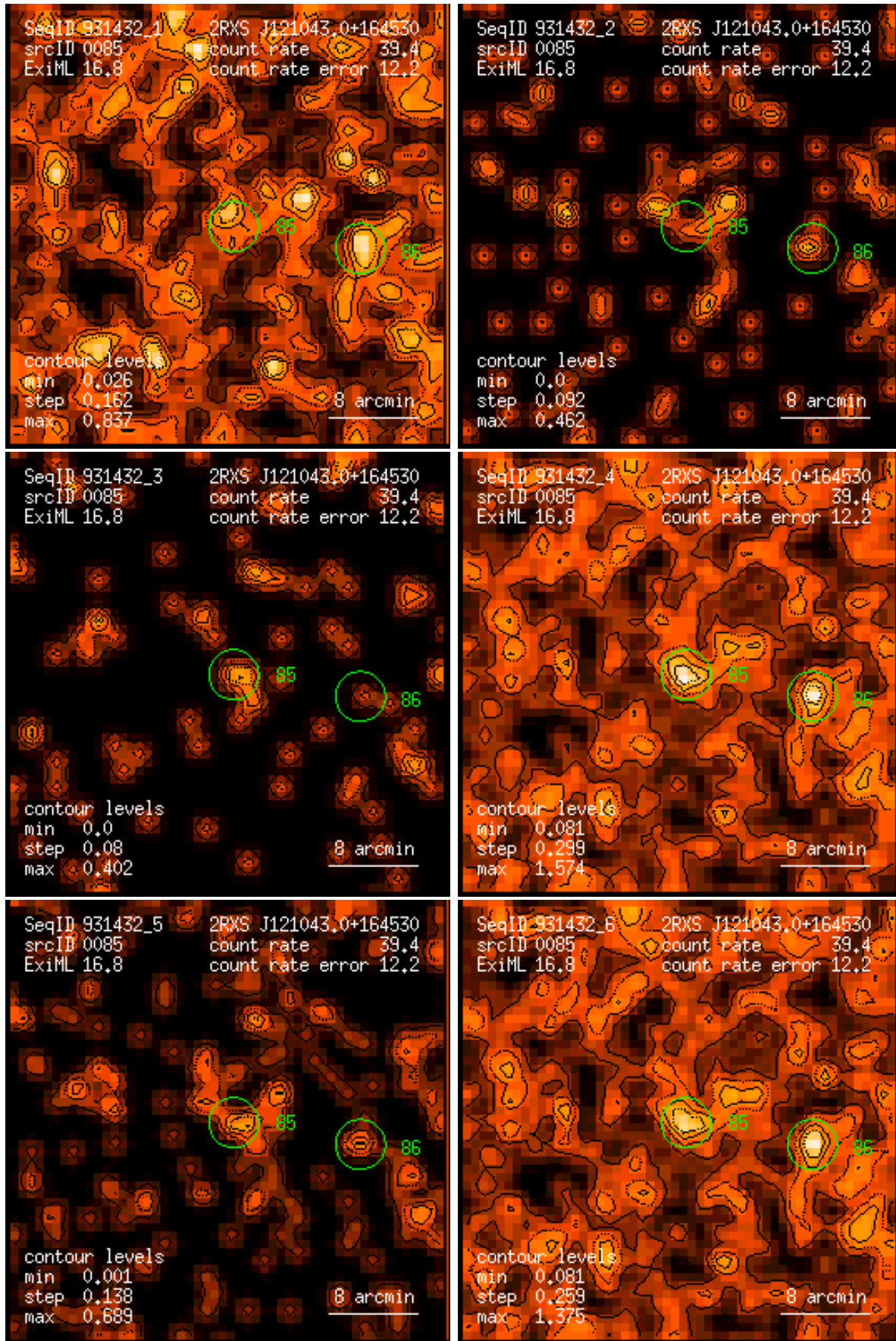
Figure 85: RASS 931432: detection 0085: band rate images, Gaussian filter: (1) PSPC channels 11 – 41, (2) 52 – 90, (3) 91 – 201, (4) 11 – 235, (5) 52 – 201, (6) 11 – 201. Broad band rates in counts/ks. Band rate contour levels in counts/ks/arcmin 2 .
