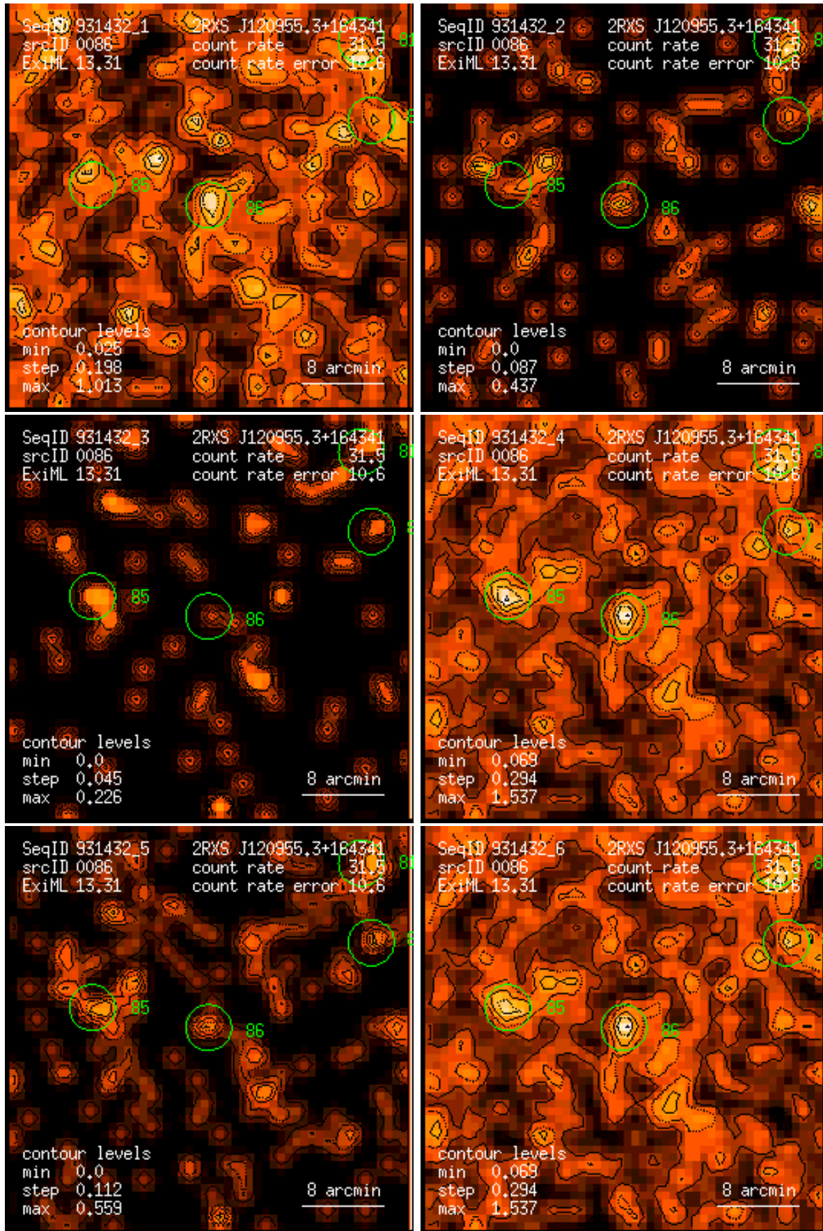
Figure 86: RASS 931432: detection 0086: band rate images, Gaussian filter: (1) PSPC channels 11 – 41, (2) 52 – 90, (3) 91 – 201, (4) 11 – 235, (5) 52 – 201, (6) 11 – 201. Broad band rates in counts/ks. Band rate contour levels in counts/ks/arcmin 2 .
