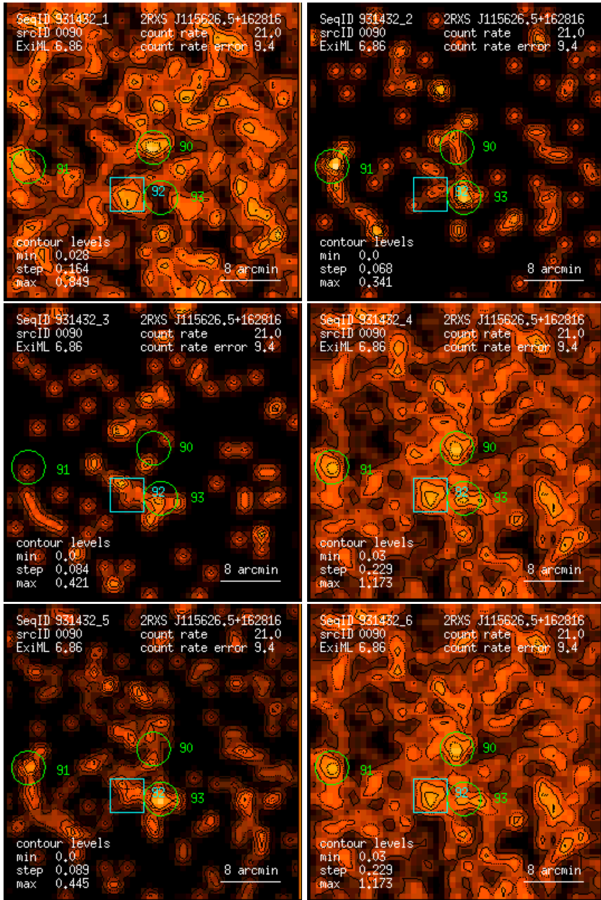
Figure 90: RASS 931432: detection 0090: band rate images, Gaussian filter: (1) PSPC channels 11 – 41, (2) 52 – 90, (3) 91 – 201, (4) 11 – 235, (5) 52 – 201, (6) 11 – 201. Broad band rates in counts/ks. Band rate contour levels in counts/ks/arcmin 2 .
