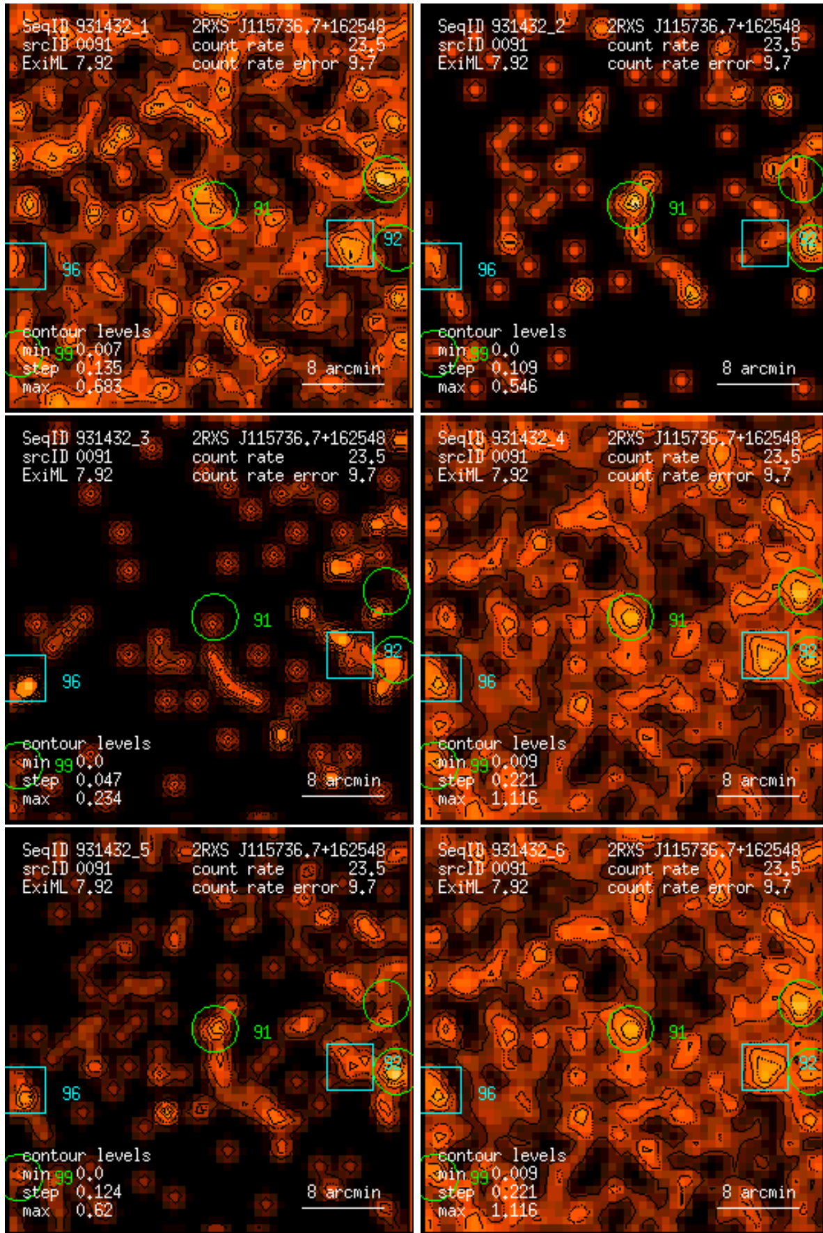
Figure 91: RASS 931432: detection 0091: band rate images, Gaussian filter: (1) PSPC channels 11 – 41, (2) 52 – 90, (3) 91 – 201, (4) 11 – 235, (5) 52 – 201, (6) 11 – 201. Broad band rates in counts/ks. Band rate contour levels in counts/ks/arcmin 2 .
