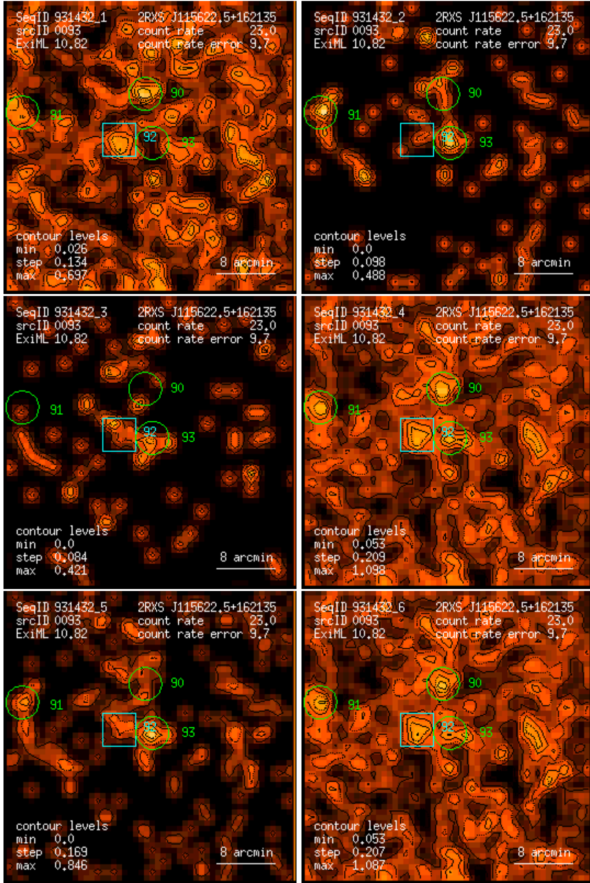
Figure 93: RASS 931432: detection 0093: band rate images, Gaussian filter: (1) PSPC channels 11 – 41, (2) 52 – 90, (3) 91 – 201, (4) 11 – 235, (5) 52 – 201, (6) 11 – 201. Broad band rates in counts/ks. Band rate contour levels in counts/ks/arcmin 2 .
