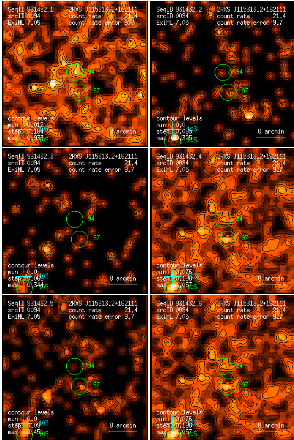
Figure 94: RASS 931432: detection 0094: band rate images, Gaussian filter: (1) PSPC channels 11 – 41, (2) 52 – 90, (3) 91 – 201, (4) 11 – 235, (5) 52 – 201, (6) 11 – 201. Broad band rates in counts/ks. Band rate contour levels in counts/ks/arcmin 2 .
