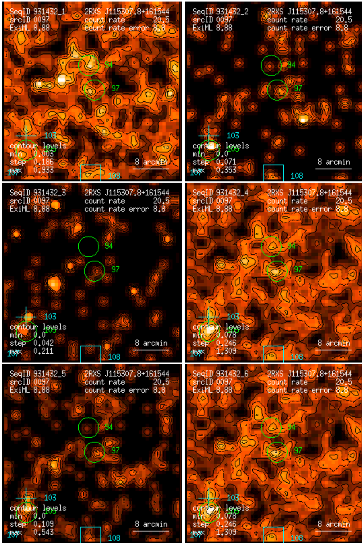
Figure 97: RASS 931432: detection 0097: band rate images, Gaussian filter: (1) PSPC channels 11 – 41, (2) 52 – 90, (3) 91 – 201, (4) 11 – 235, (5) 52 – 201, (6) 11 – 201. Broad band rates in counts/ks. Band rate contour levels in counts/ks/arcmin 2 .
