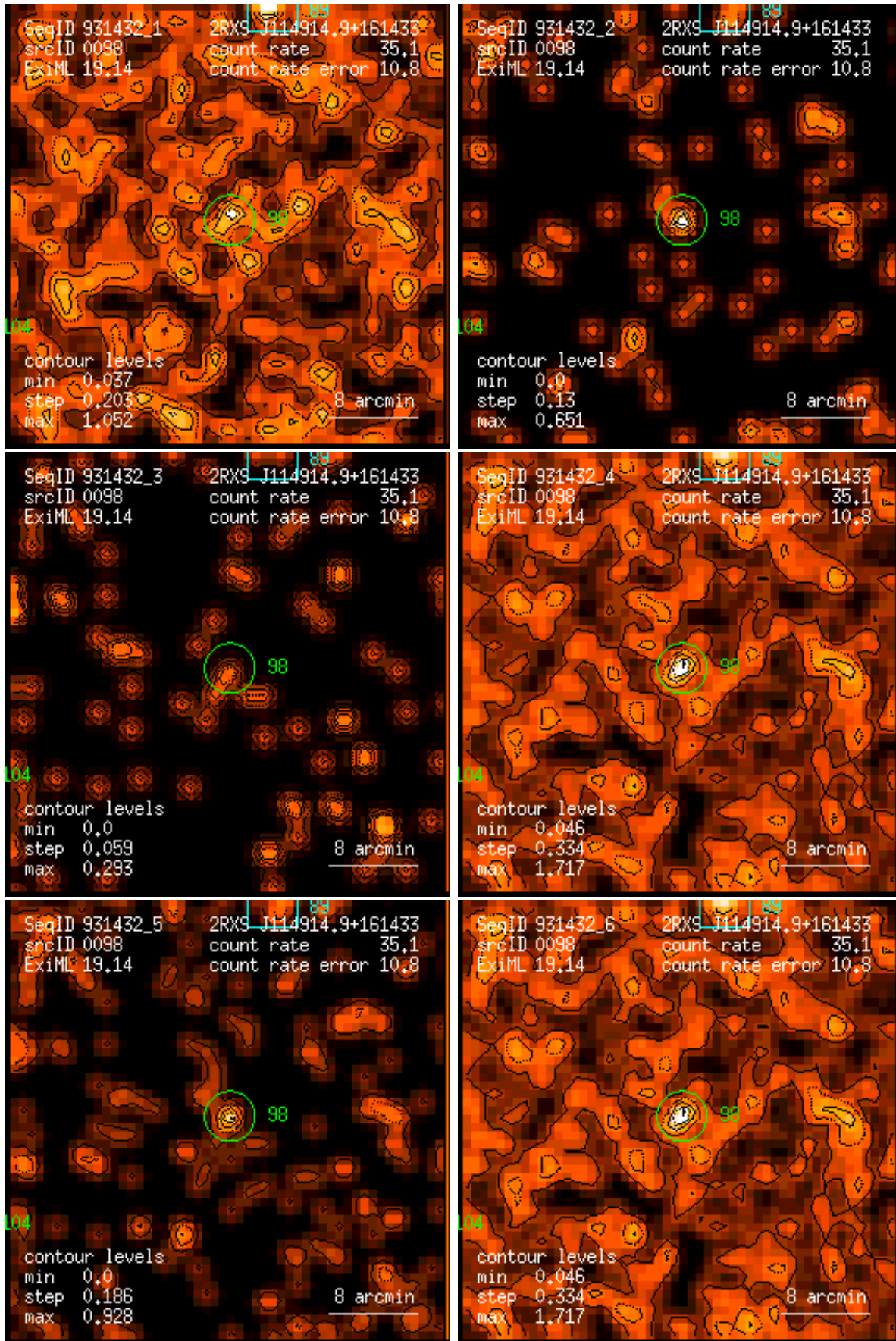
Figure 98: RASS 931432: detection 0098: band rate images, Gaussian filter: (1) PSPC channels 11 – 41, (2) 52 – 90, (3) 91 – 201, (4) 11 – 235, (5) 52 – 201, (6) 11 – 201. Broad band rates in counts/ks. Band rate contour levels in counts/ks/arcmin 2 .
