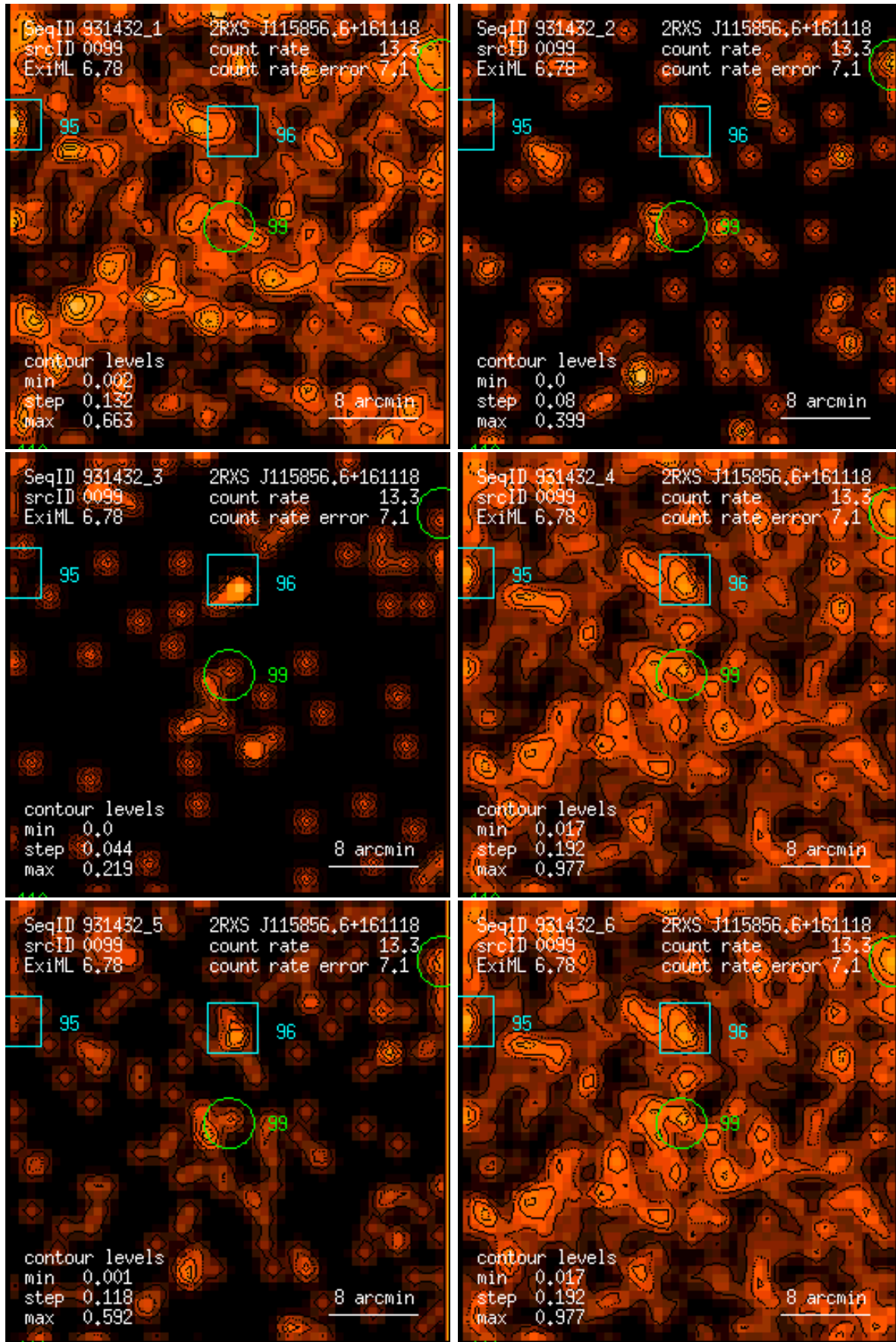
Figure 99: RASS 931432: detection 0099: band rate images, Gaussian filter: (1) PSPC channels 11 – 41, (2) 52 – 90, (3) 91 – 201, (4) 11 – 235, (5) 52 – 201, (6) 11 – 201. Broad band rates in counts/ks. Band rate contour levels in counts/ks/arcmin 2 .
