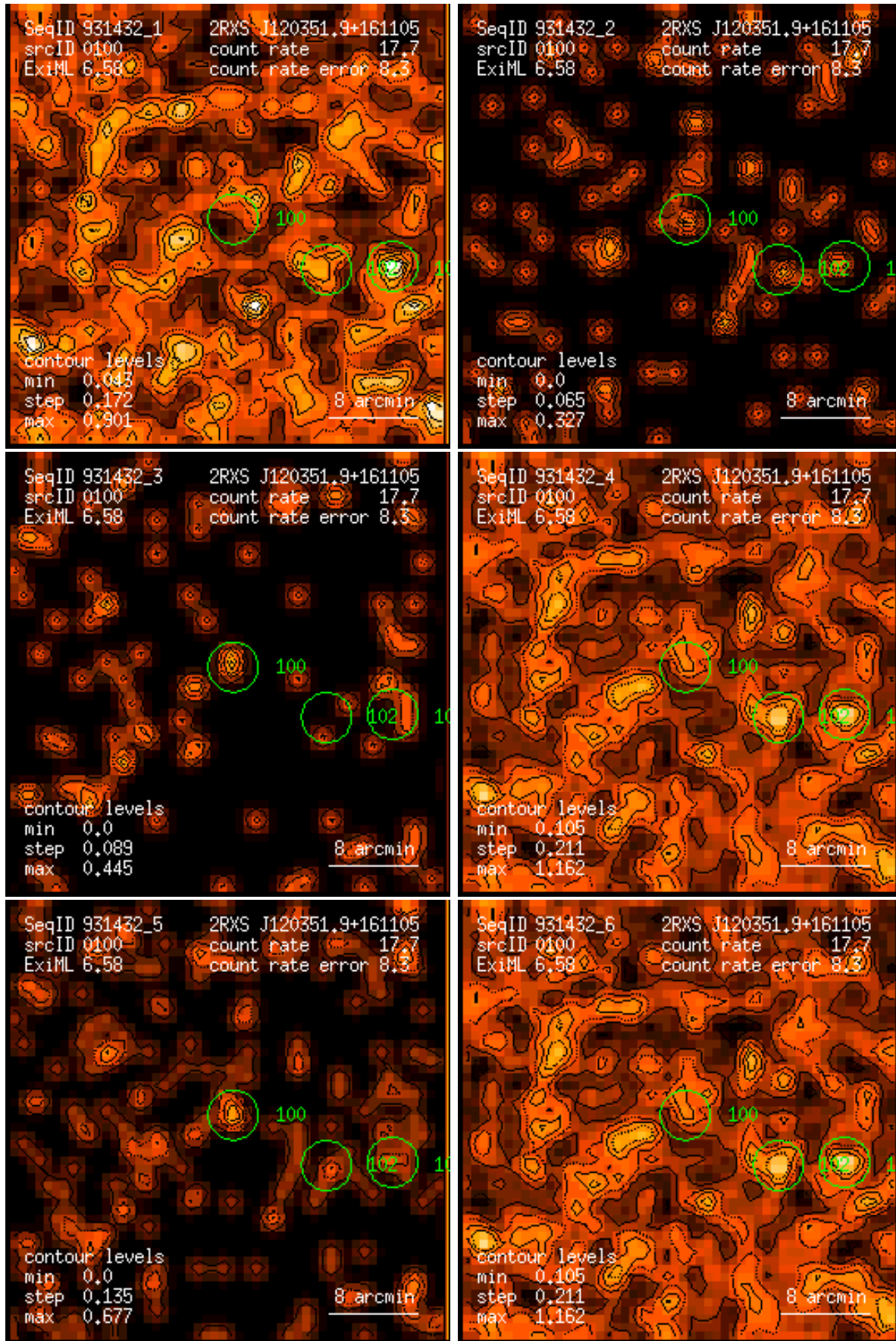
Figure 100: RASS 931432: detection 0100: band rate images, Gaussian filter: (1) PSPC channels 11 – 41, (2) 52 – 90, (3) 91 – 201, (4) 11 – 235, (5) 52 – 201, (6) 11 – 201. Broad band rates in counts/ks. Band rate contour levels in counts/ks/arcmin 2 .
