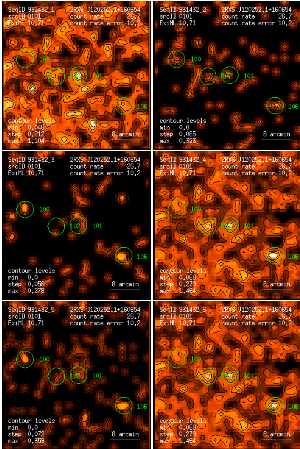
Figure 101: RASS 931432: detection 0101: band rate images, Gaussian filter: (1) PSPC channels 11 – 41, (2) 52 – 90, (3) 91 – 201, (4) 11 – 235, (5) 52 – 201, (6) 11 – 201. Broad band rates in counts/ks. Band rate contour levels in counts/ks/arcmin 2 .
