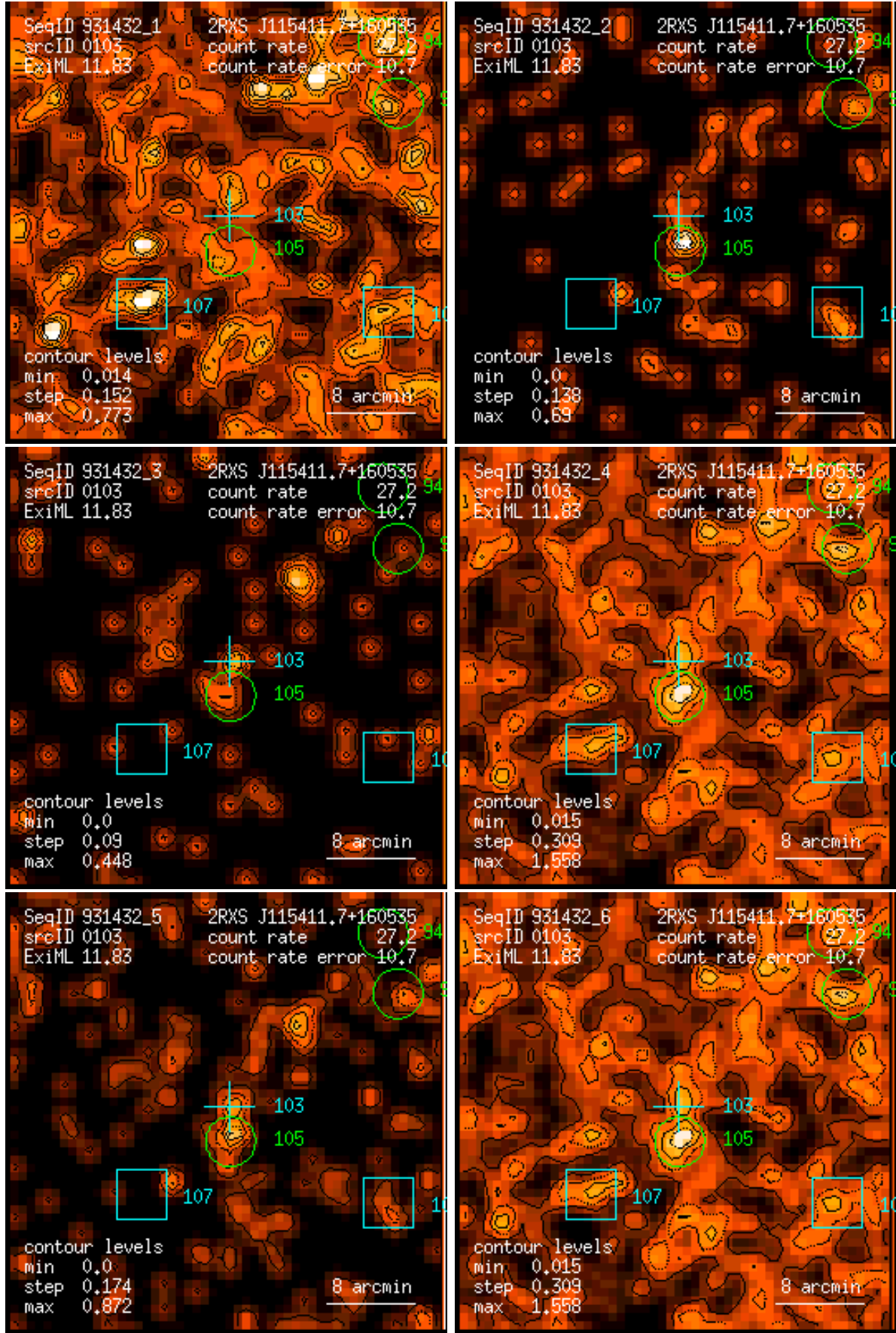
Figure 103: RASS 931432: detection 0103: band rate images, Gaussian filter: (1) PSPC channels 11 – 41, (2) 52 – 90, (3) 91 – 201, (4) 11 – 235, (5) 52 – 201, (6) 11 – 201. Broad band rates in counts/ks. Band rate contour levels in counts/ks/arcmin 2 .
