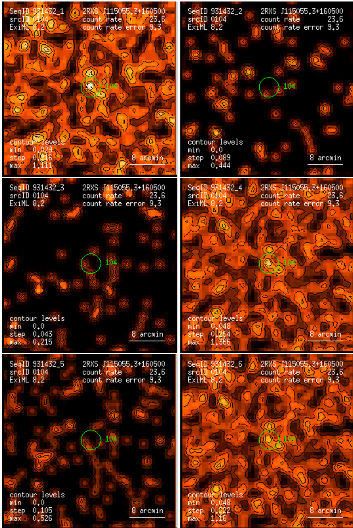
Figure 104: RASS 931432: detection 0104: band rate images, Gaussian filter: (1) PSPC channels 11 – 41, (2) 52 – 90, (3) 91 – 201, (4) 11 – 235, (5) 52 – 201, (6) 11 – 201. Broad band rates in counts/ks. Band rate contour levels in counts/ks/arcmin 2 .
