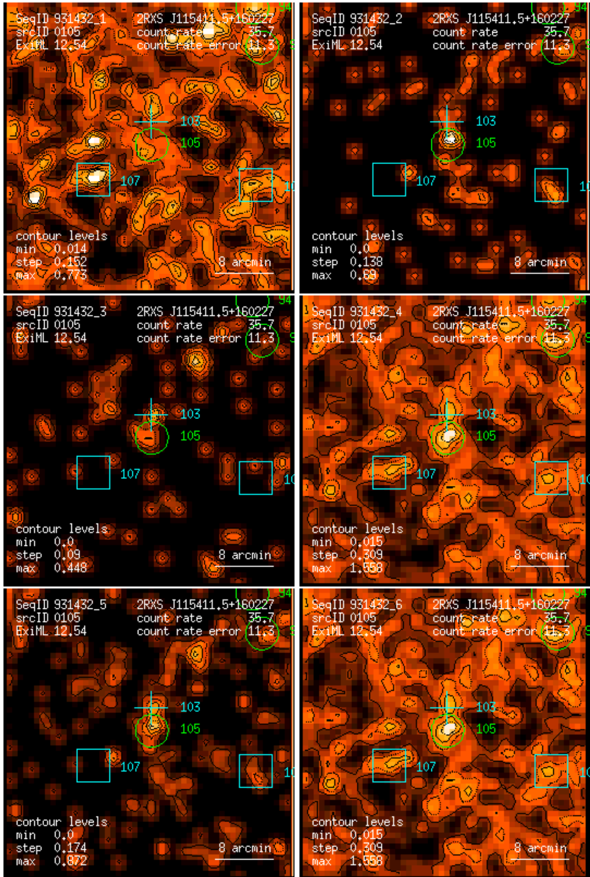
Figure 105: RASS 931432: detection 0105: band rate images, Gaussian filter: (1) PSPC channels 11 – 41, (2) 52 – 90, (3) 91 – 201, (4) 11 – 235, (5) 52 – 201, (6) 11 – 201. Broad band rates in counts/ks. Band rate contour levels in counts/ks/arcmin 2 .
