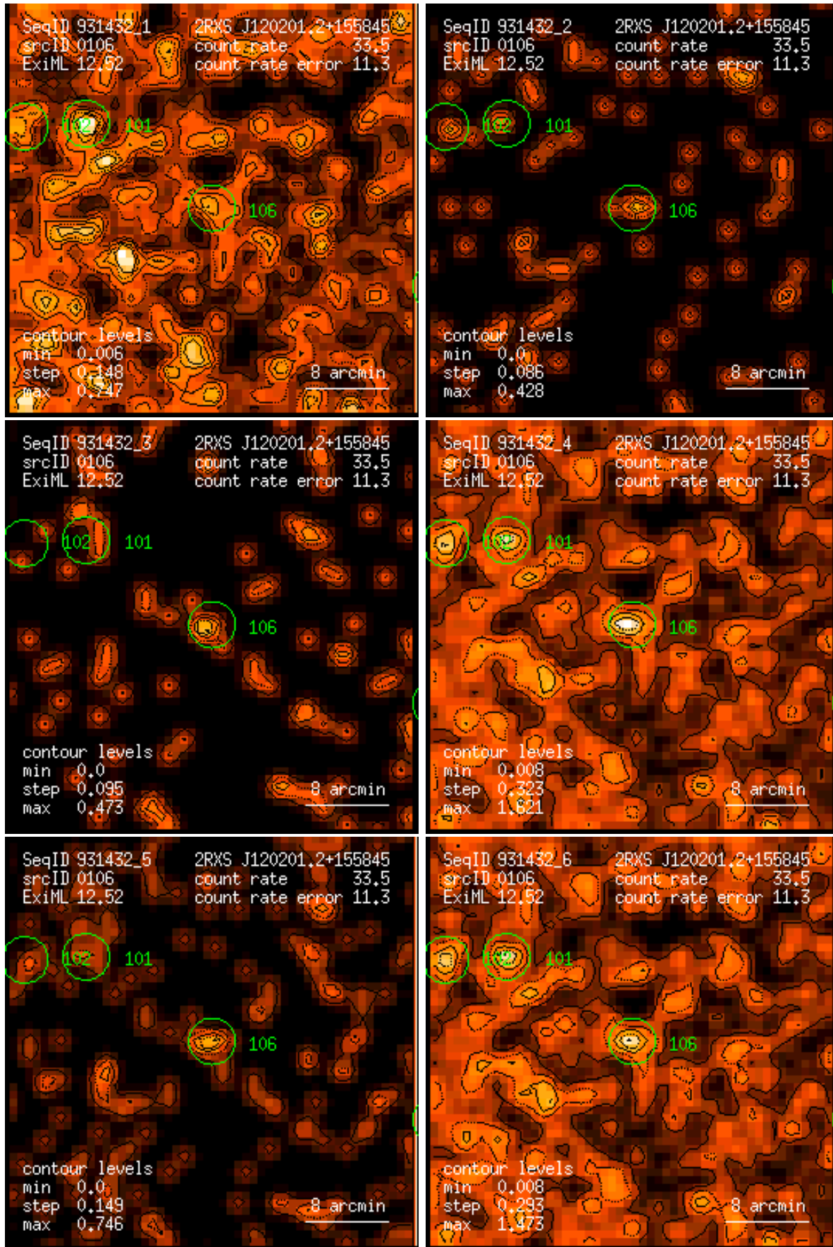
Figure 106: RASS 931432: detection 0106: band rate images, Gaussian filter: (1) PSPC channels 11 – 41, (2) 52 – 90, (3) 91 – 201, (4) 11 – 235, (5) 52 – 201, (6) 11 – 201. Broad band rates in counts/ks. Band rate contour levels in counts/ks/arcmin 2 .
