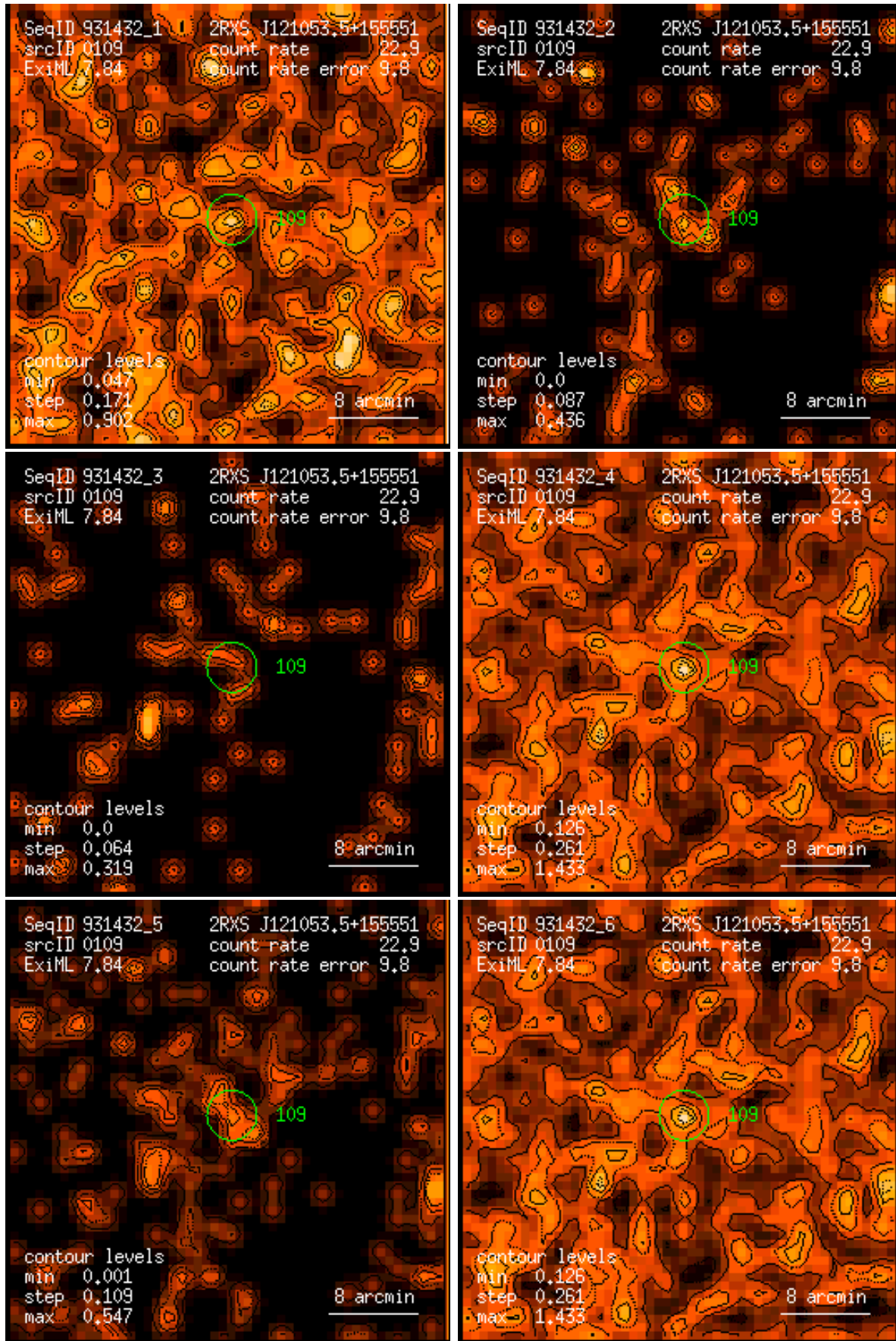
Figure 109: RASS 931432: detection 0109: band rate images, Gaussian filter: (1) PSPC channels 11 – 41, (2) 52 – 90, (3) 91 – 201, (4) 11 – 235, (5) 52 – 201, (6) 11 – 201. Broad band rates in counts/ks. Band rate contour levels in counts/ks/arcmin 2 .
