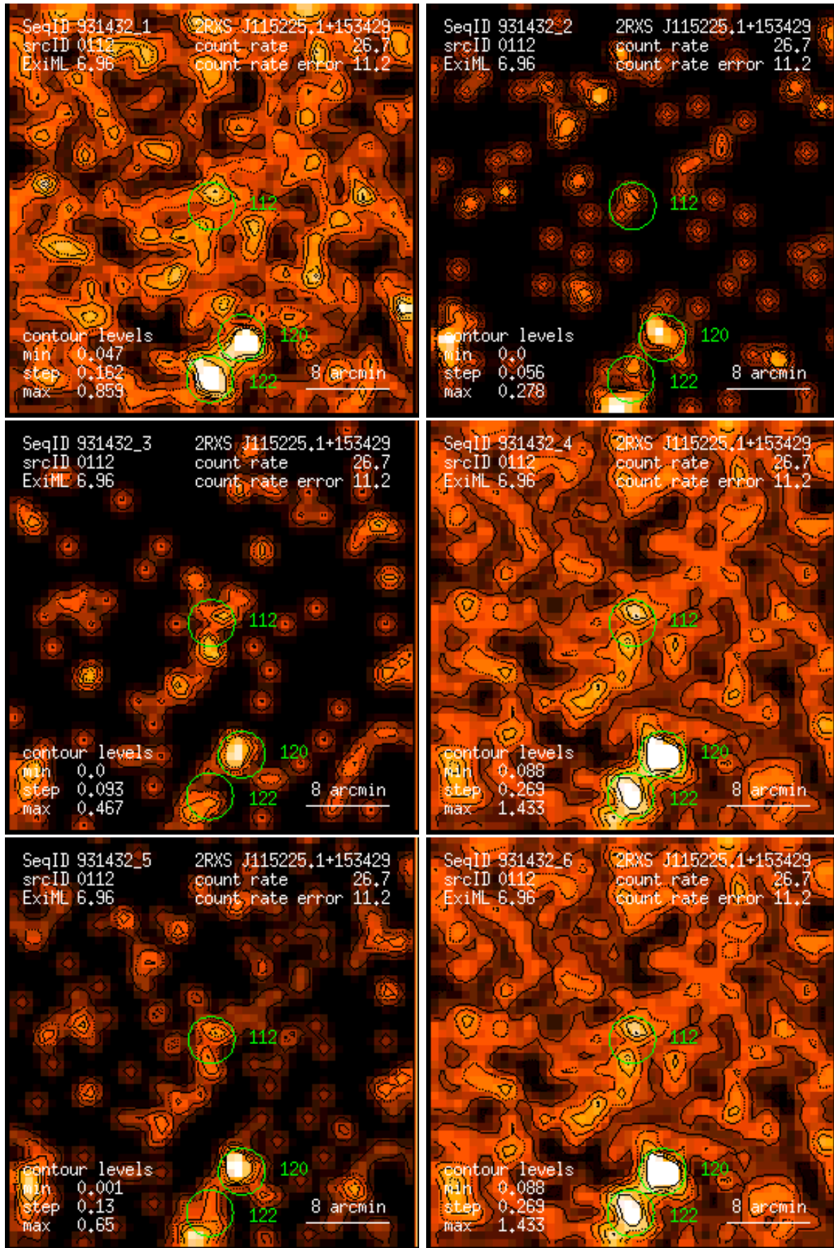
Figure 112: RASS 931432: detection 0112: band rate images, Gaussian filter: (1) PSPC channels 11 – 41, (2) 52 – 90, (3) 91 – 201, (4) 11 – 235, (5) 52 – 201, (6) 11 – 201. Broad band rates in counts/ks. Band rate contour levels in counts/ks/arcmin 2 .
