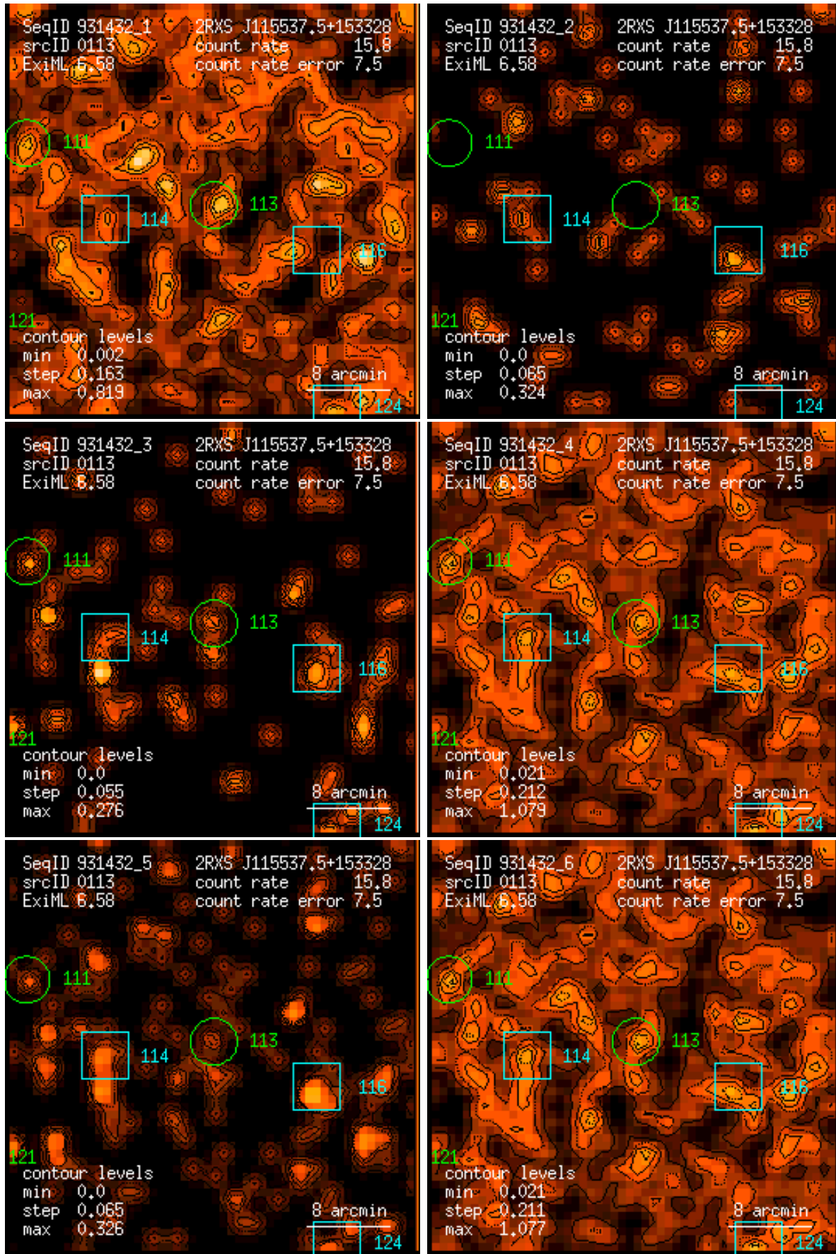
Figure 113: RASS 931432: detection 0113: band rate images, Gaussian filter: (1) PSPC channels 11 – 41, (2) 52 – 90, (3) 91 – 201, (4) 11 – 235, (5) 52 – 201, (6) 11 – 201. Broad band rates in counts/ks. Band rate contour levels in counts/ks/arcmin 2 .
