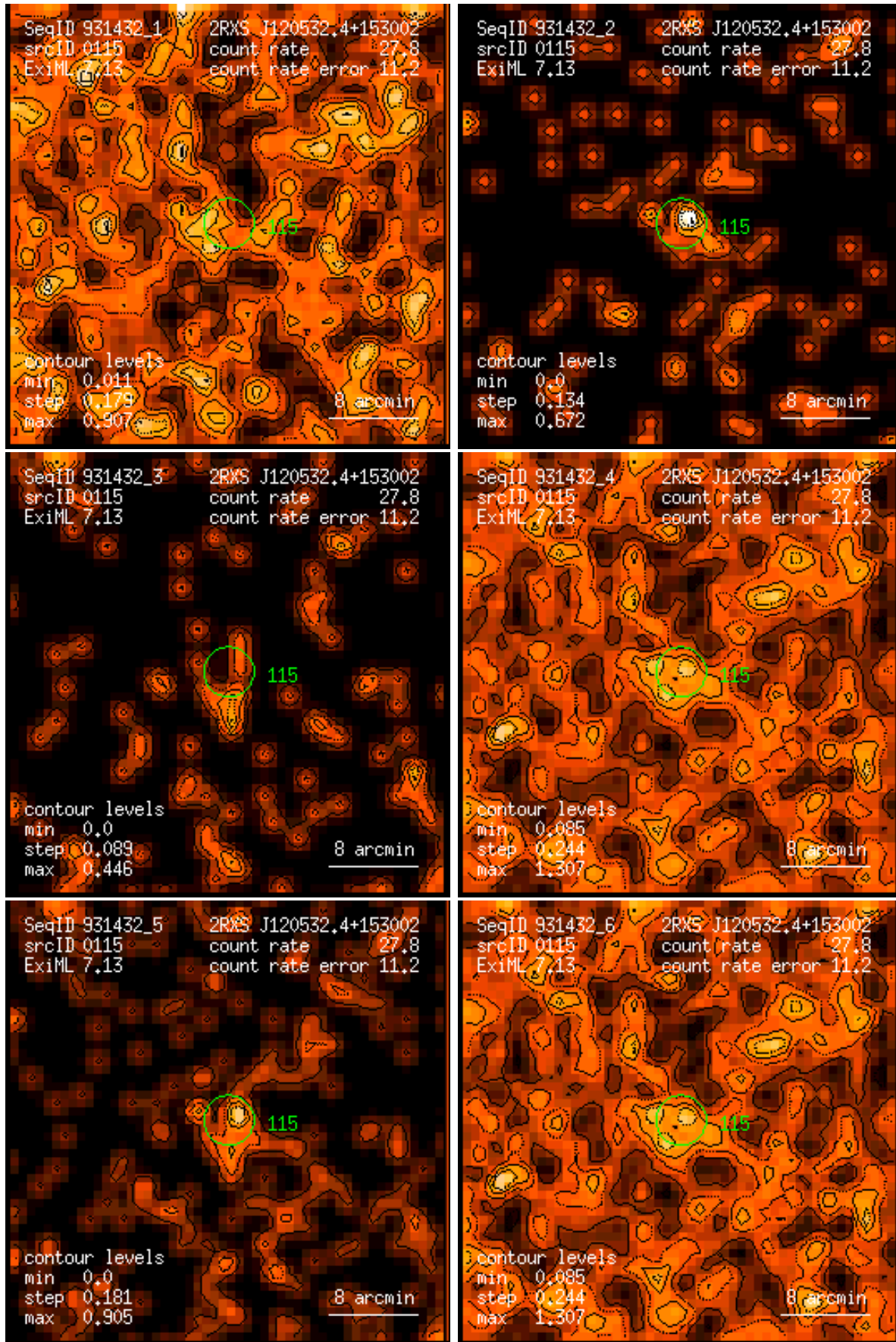
Figure 115: RASS 931432: detection 0115: band rate images, Gaussian filter: (1) PSPC channels 11 – 41, (2) 52 – 90, (3) 91 – 201, (4) 11 – 235, (5) 52 – 201, (6) 11 – 201. Broad band rates in counts/ks. Band rate contour levels in counts/ks/arcmin 2 .
