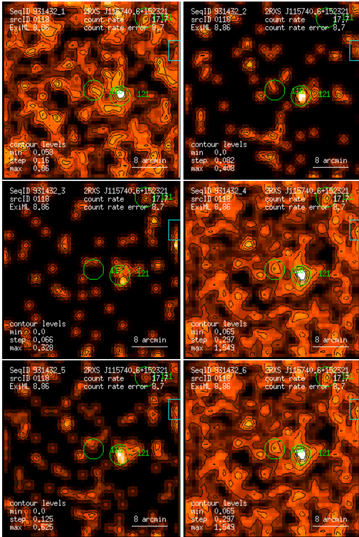
Figure 118: RASS 931432: detection 0118: band rate images, Gaussian filter: (1) PSPC channels 11 – 41, (2) 52 – 90, (3) 91 – 201, (4) 11 – 235, (5) 52 – 201, (6) 11 – 201. Broad band rates in counts/ks. Band rate contour levels in counts/ks/arcmin 2 .
