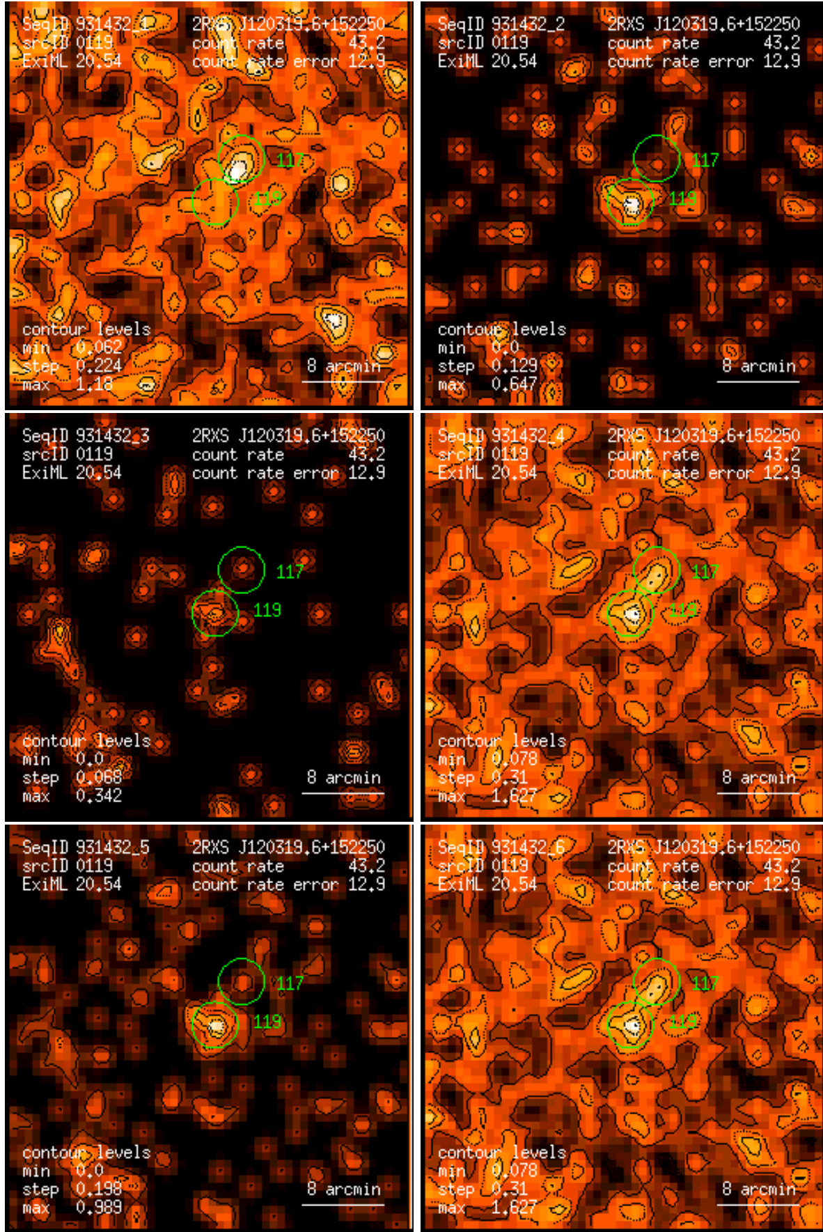
Figure 119: RASS 931432: detection 0119: band rate images, Gaussian filter: (1) PSPC channels 11 – 41, (2) 52 – 90, (3) 91 – 201, (4) 11 – 235, (5) 52 – 201, (6) 11 – 201. Broad band rates in counts/ks. Band rate contour levels in counts/ks/arcmin 2 .
