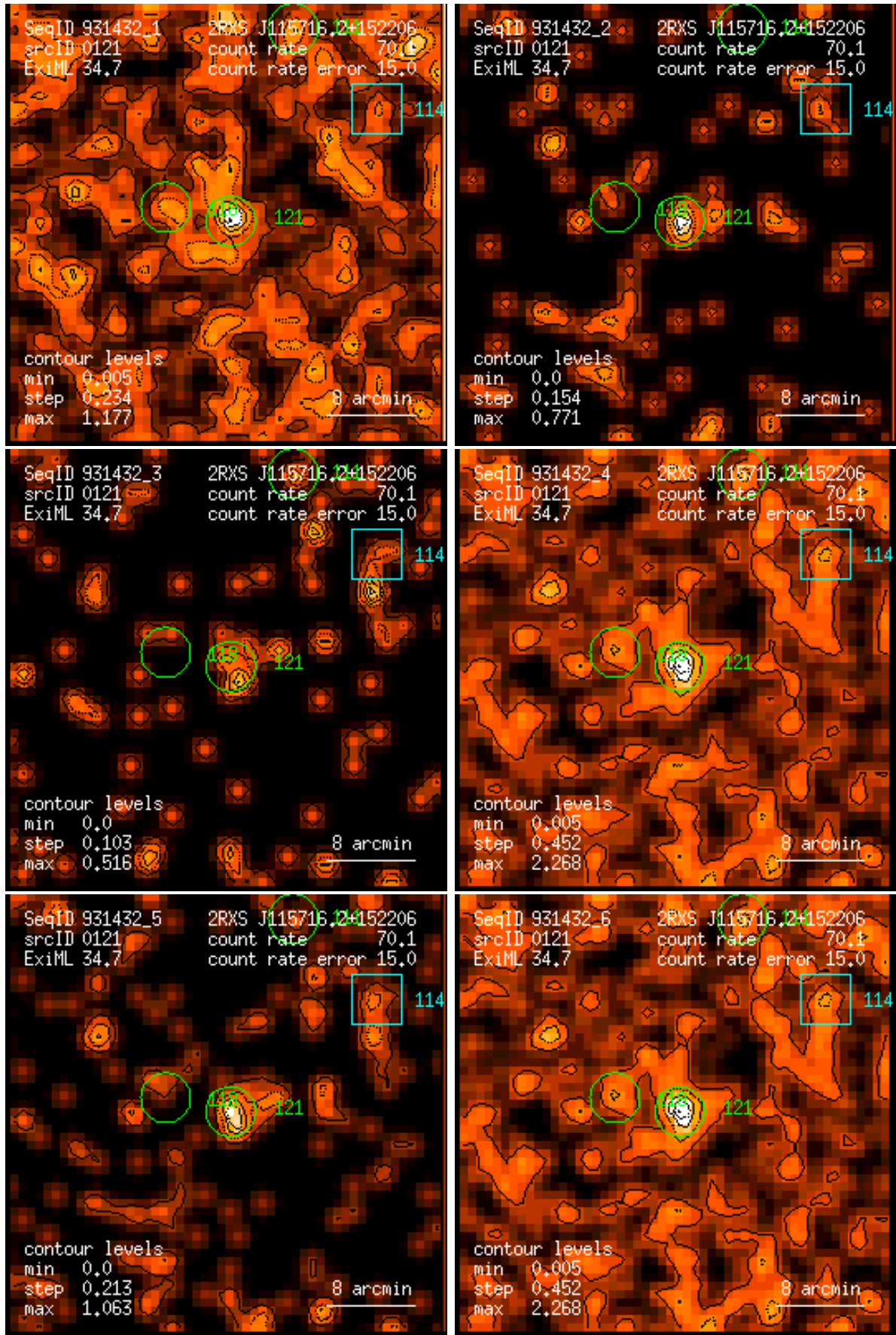
Figure 121: RASS 931432: detection 0121: band rate images, Gaussian filter: (1) PSPC channels 11 – 41, (2) 52 – 90, (3) 91 – 201, (4) 11 – 235, (5) 52 – 201, (6) 11 – 201. Broad band rates in counts/ks. Band rate contour levels in counts/ks/arcmin 2 .
