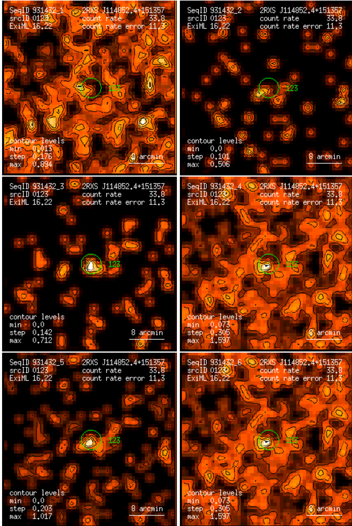
Figure 123: RASS 931432: detection 0123: band rate images, Gaussian filter: (1) PSPC channels 11 – 41, (2) 52 – 90, (3) 91 – 201, (4) 11 – 235, (5) 52 – 201, (6) 11 – 201. Broad band rates in counts/ks. Band rate contour levels in counts/ks/arcmin 2 .
