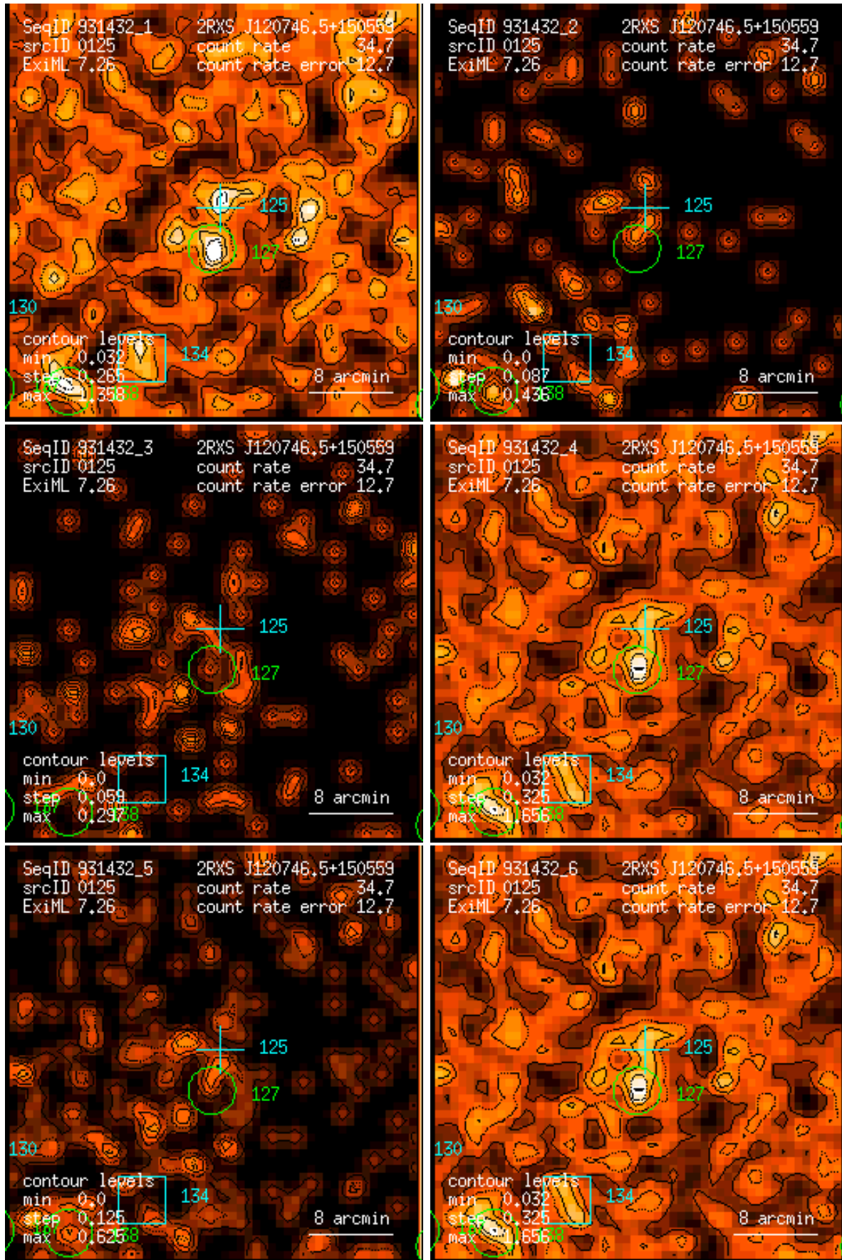
Figure 125: RASS 931432: detection 0125: band rate images, Gaussian filter: (1) PSPC channels 11 – 41, (2) 52 – 90, (3) 91 – 201, (4) 11 – 235, (5) 52 – 201, (6) 11 – 201. Broad band rates in counts/ks. Band rate contour levels in counts/ks/arcmin 2 .
