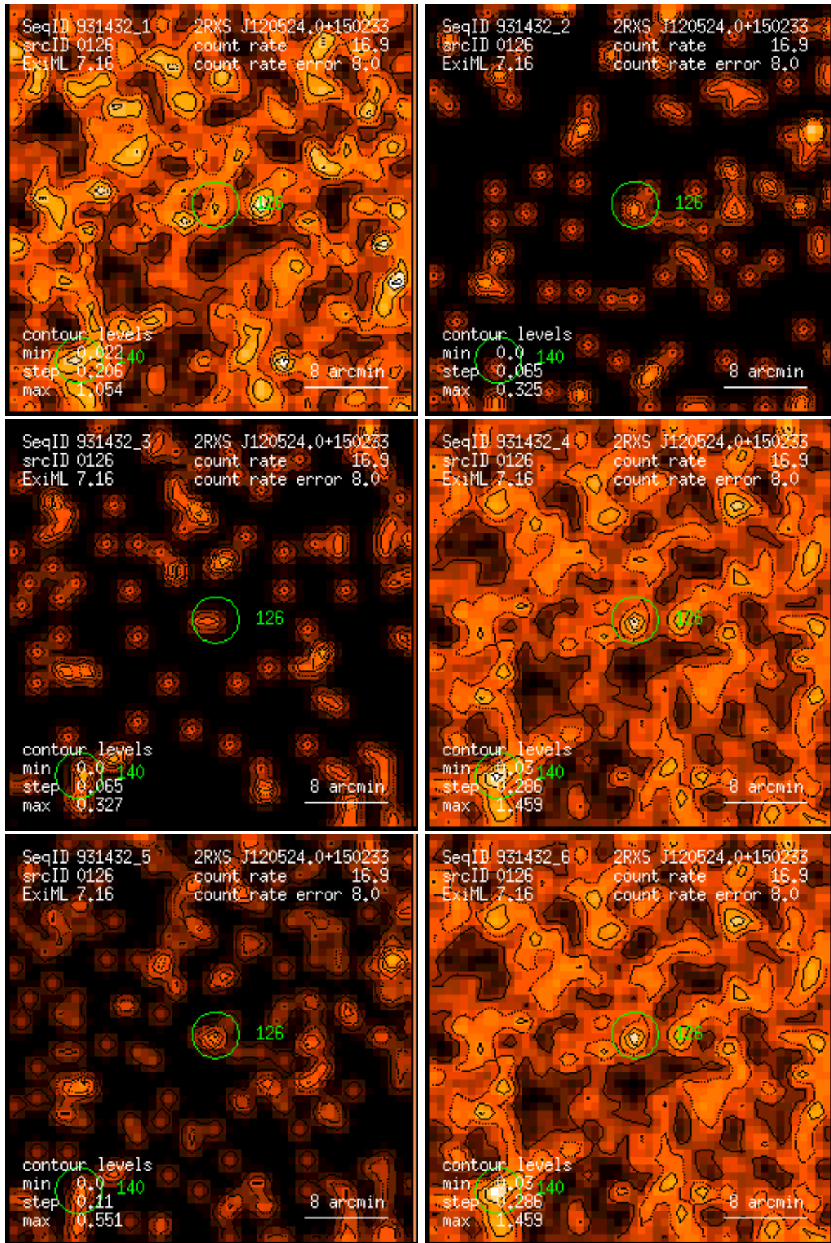
Figure 126: RASS 931432: detection 0126: band rate images, Gaussian filter: (1) PSPC channels 11 – 41, (2) 52 – 90, (3) 91 – 201, (4) 11 – 235, (5) 52 – 201, (6) 11 – 201. Broad band rates in counts/ks. Band rate contour levels in counts/ks/arcmin 2 .
