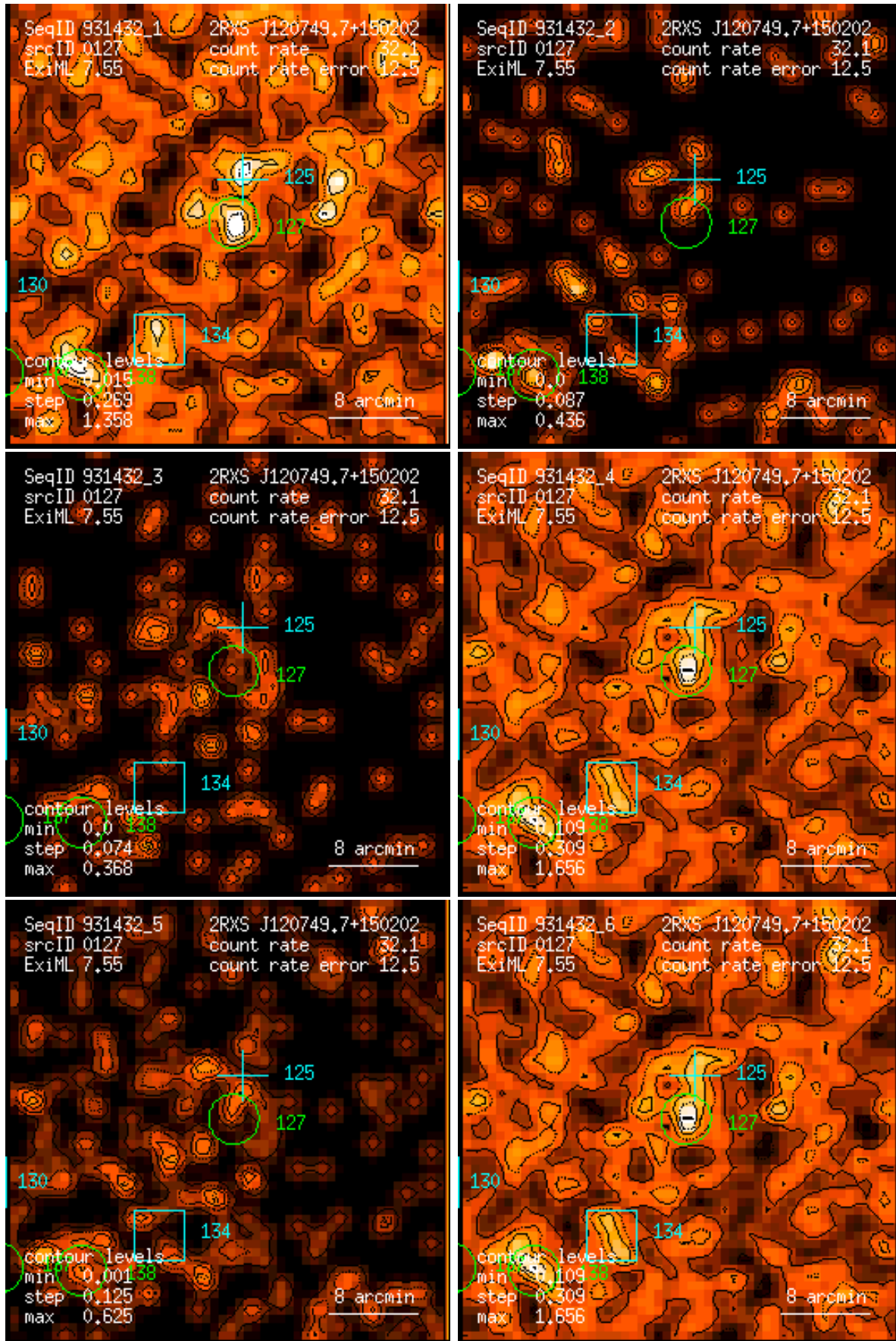
Figure 127: RASS 931432: detection 0127: band rate images, Gaussian filter: (1) PSPC channels 11 – 41, (2) 52 – 90, (3) 91 – 201, (4) 11 – 235, (5) 52 – 201, (6) 11 – 201. Broad band rates in counts/ks. Band rate contour levels in counts/ks/arcmin 2 .
