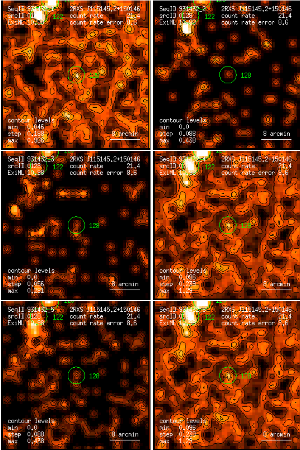
Figure 128: RASS 931432: detection 0128: band rate images, Gaussian filter: (1) PSPC channels 11 – 41, (2) 52 – 90, (3) 91 – 201, (4) 11 – 235, (5) 52 – 201, (6) 11 – 201. Broad band rates in counts/ks. Band rate contour levels in counts/ks/arcmin 2 .
