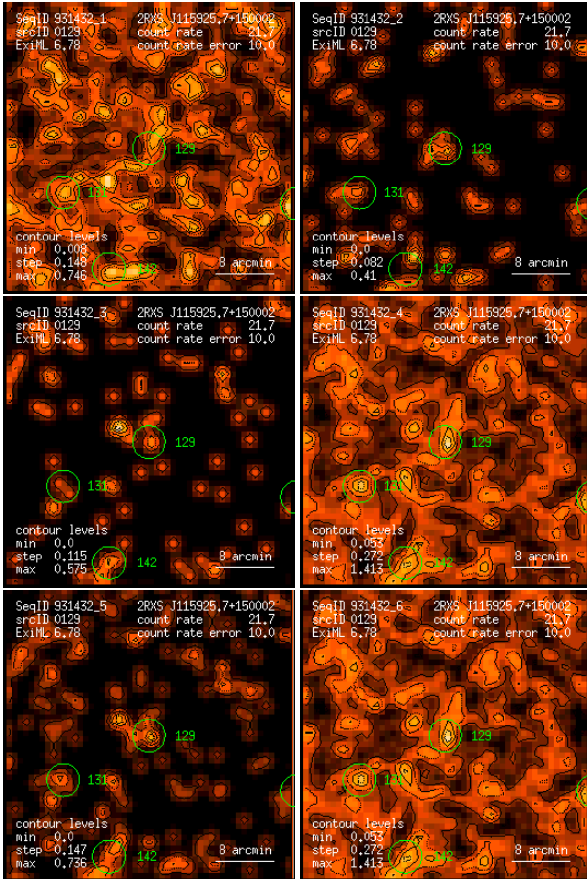
Figure 129: RASS 931432: detection 0129: band rate images, Gaussian filter: (1) PSPC channels 11 – 41, (2) 52 – 90, (3) 91 – 201, (4) 11 – 235, (5) 52 – 201, (6) 11 – 201. Broad band rates in counts/ks. Band rate contour levels in counts/ks/arcmin 2 .
