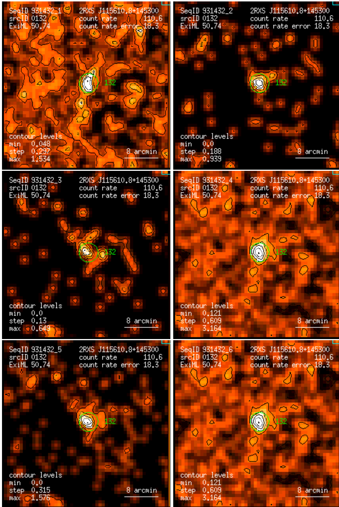
Figure 132: RASS 931432: detection 0132: band rate images, Gaussian filter: (1) PSPC channels 11 – 41, (2) 52 – 90, (3) 91 – 201, (4) 11 – 235, (5) 52 – 201, (6) 11 – 201. Broad band rates in counts/ks. Band rate contour levels in counts/ks/arcmin 2 .
