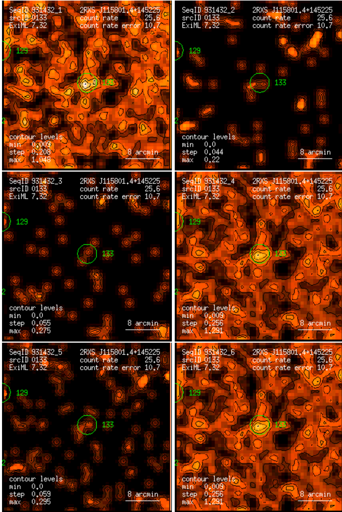
Figure 133: RASS 931432: detection 0133: band rate images, Gaussian filter: (1) PSPC channels 11 – 41, (2) 52 – 90, (3) 91 – 201, (4) 11 – 235, (5) 52 – 201, (6) 11 – 201. Broad band rates in counts/ks. Band rate contour levels in counts/ks/arcmin 2 .
