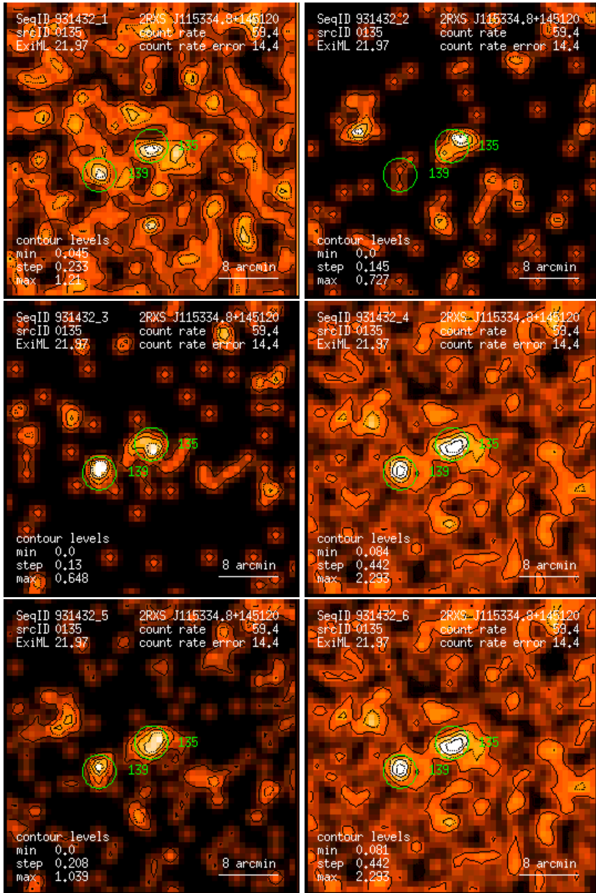
Figure 135: RASS 931432: detection 0135: band rate images, Gaussian filter: (1) PSPC channels 11 – 41, (2) 52 – 90, (3) 91 – 201, (4) 11 – 235, (5) 52 – 201, (6) 11 – 201. Broad band rates in counts/ks. Band rate contour levels in counts/ks/arcmin 2 .
