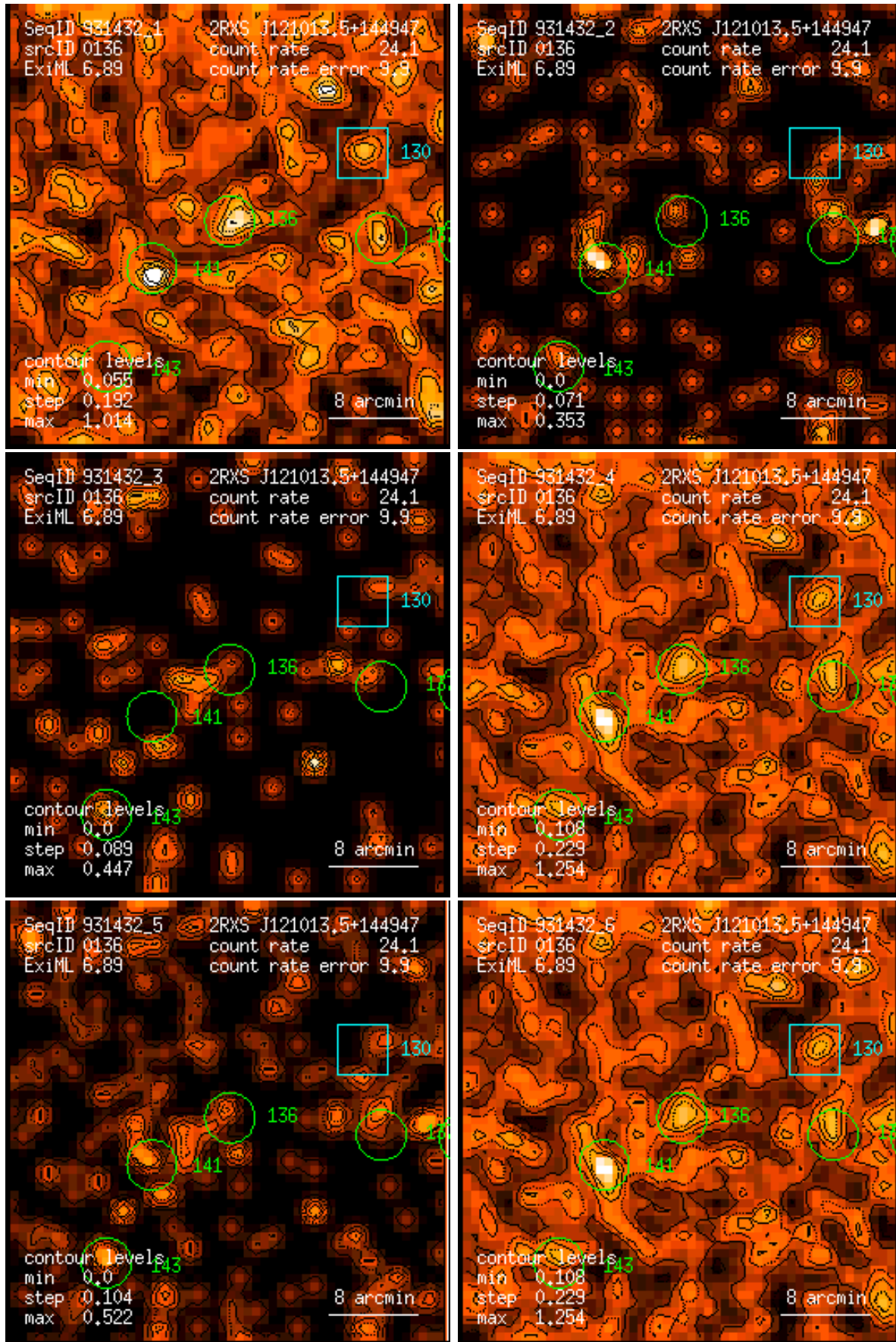
Figure 136: RASS 931432: detection 0136: band rate images, Gaussian filter: (1) PSPC channels 11 – 41, (2) 52 – 90, (3) 91 – 201, (4) 11 – 235, (5) 52 – 201, (6) 11 – 201. Broad band rates in counts/ks. Band rate contour levels in counts/ks/arcmin 2 .
