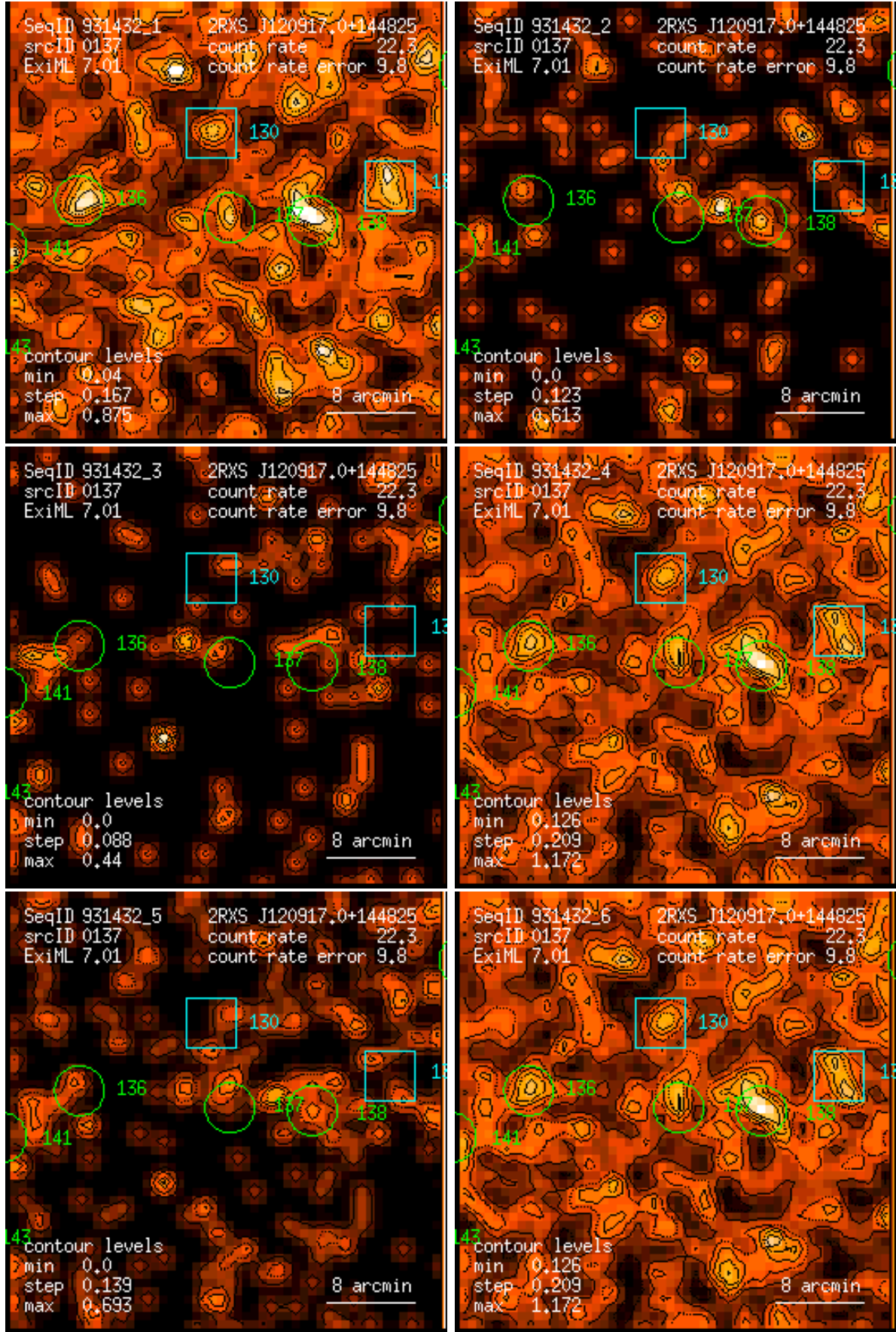
Figure 137: RASS 931432: detection 0137: band rate images, Gaussian filter: (1) PSPC channels 11 – 41, (2) 52 – 90, (3) 91 – 201, (4) 11 – 235, (5) 52 – 201, (6) 11 – 201. Broad band rates in counts/ks. Band rate contour levels in counts/ks/arcmin 2 .
