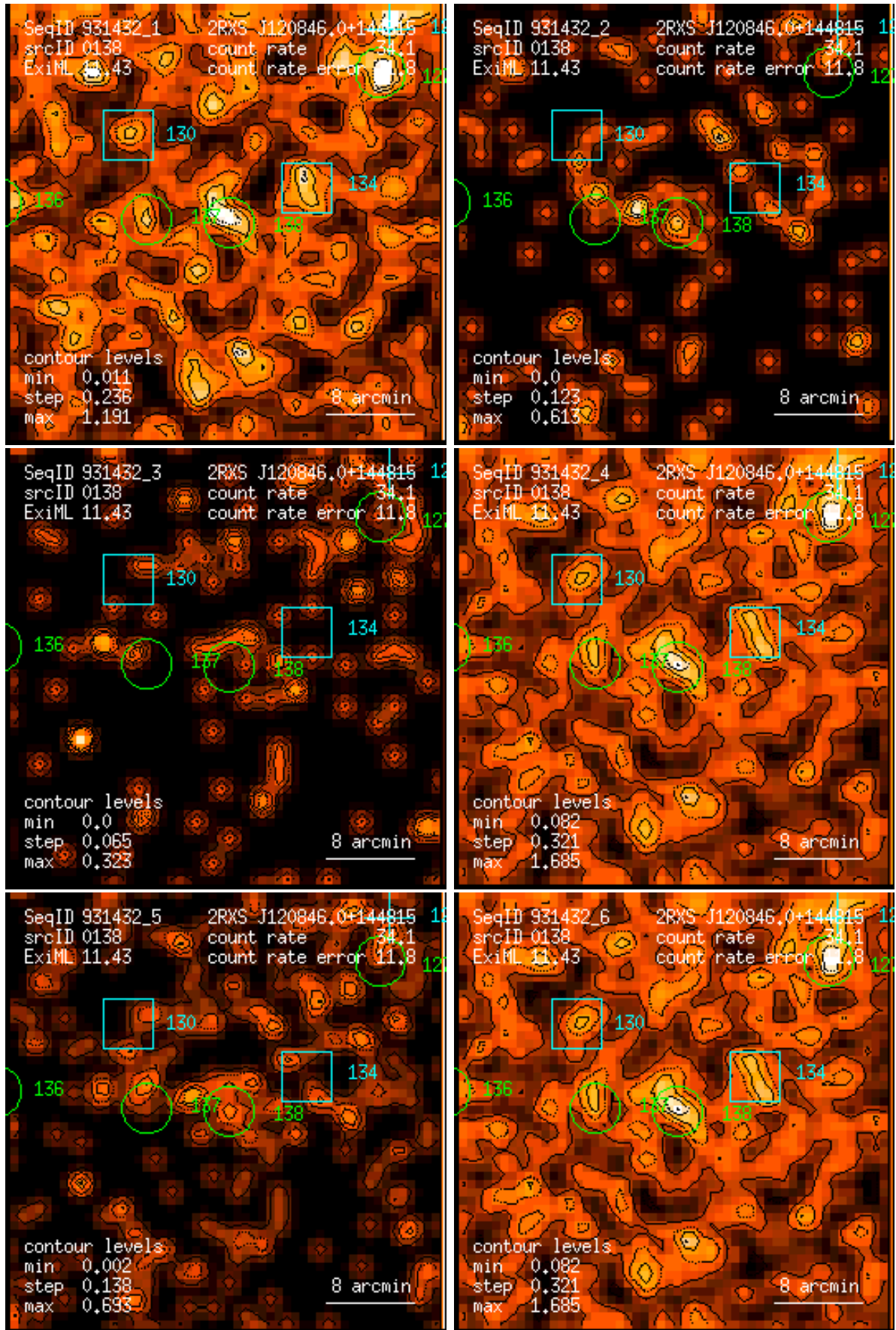
Figure 138: RASS 931432: detection 0138: band rate images, Gaussian filter: (1) PSPC channels 11 – 41, (2) 52 – 90, (3) 91 – 201, (4) 11 – 235, (5) 52 – 201, (6) 11 – 201. Broad band rates in counts/ks. Band rate contour levels in counts/ks/arcmin 2 .
