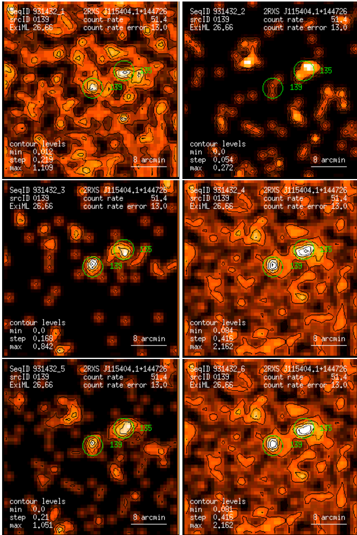
Figure 139: RASS 931432: detection 0139: band rate images, Gaussian filter: (1) PSPC channels 11 – 41, (2) 52 – 90, (3) 91 – 201, (4) 11 – 235, (5) 52 – 201, (6) 11 – 201. Broad band rates in counts/ks. Band rate contour levels in counts/ks/arcmin 2 .
