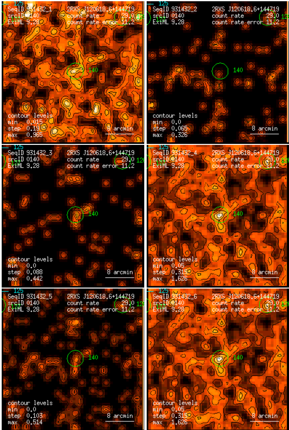
Figure 140: RASS 931432: detection 0140: band rate images, Gaussian filter: (1) PSPC channels 11 – 41, (2) 52 – 90, (3) 91 – 201, (4) 11 – 235, (5) 52 – 201, (6) 11 – 201. Broad band rates in counts/ks. Band rate contour levels in counts/ks/arcmin 2 .
