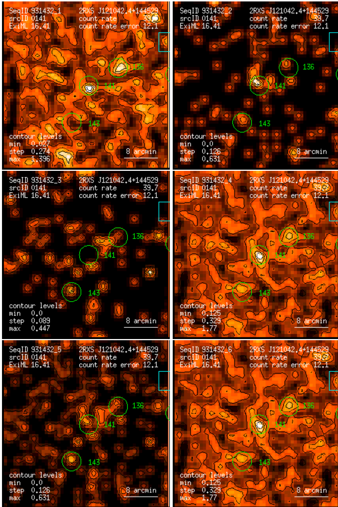
Figure 141: RASS 931432: detection 0141: band rate images, Gaussian filter: (1) PSPC channels 11 – 41, (2) 52 – 90, (3) 91 – 201, (4) 11 – 235, (5) 52 – 201, (6) 11 – 201. Broad band rates in counts/ks. Band rate contour levels in counts/ks/arcmin 2 .
