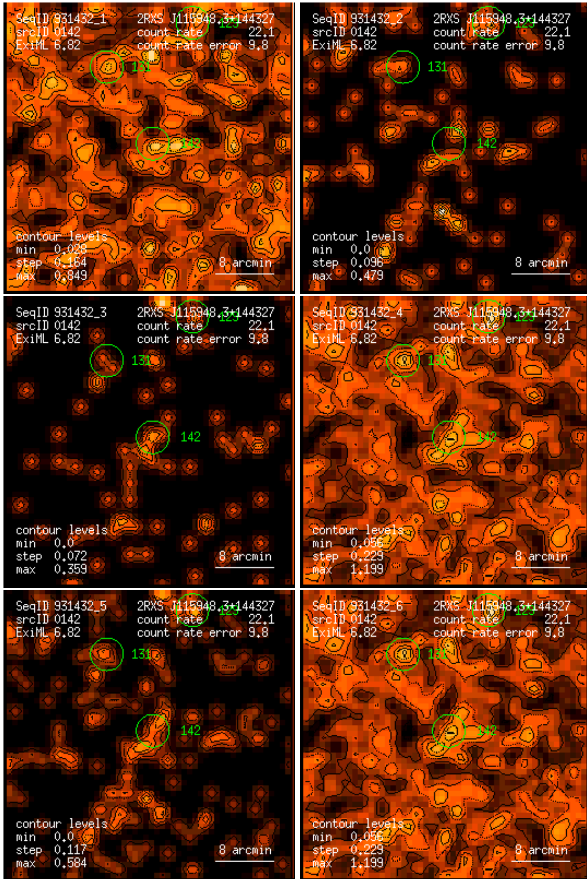
Figure 142: RASS 931432: detection 0142: band rate images, Gaussian filter: (1) PSPC channels 11 – 41, (2) 52 – 90, (3) 91 – 201, (4) 11 – 235, (5) 52 – 201, (6) 11 – 201. Broad band rates in counts/ks. Band rate contour levels in counts/ks/arcmin 2 .
