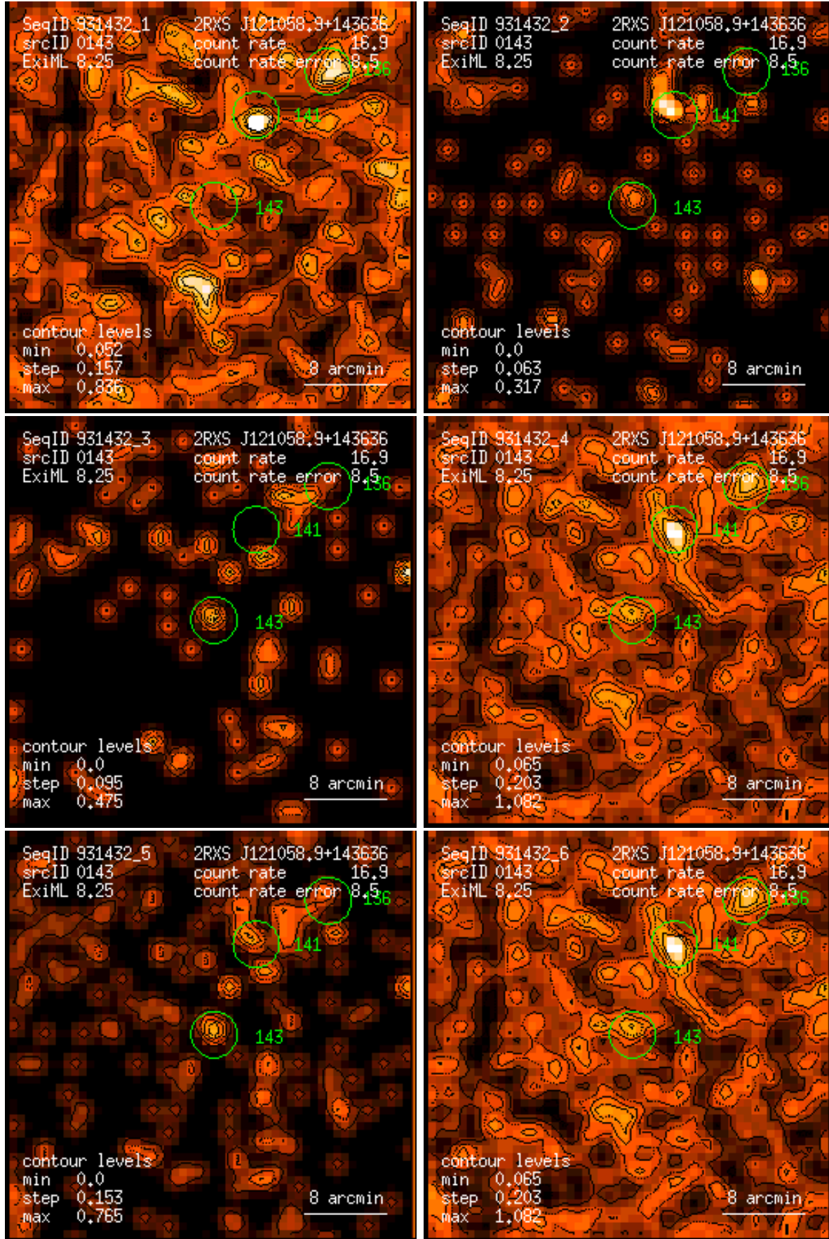
Figure 143: RASS 931432: detection 0143: band rate images, Gaussian filter: (1) PSPC channels 11 – 41, (2) 52 – 90, (3) 91 – 201, (4) 11 – 235, (5) 52 – 201, (6) 11 – 201. Broad band rates in counts/ks. Band rate contour levels in counts/ks/arcmin 2 .
