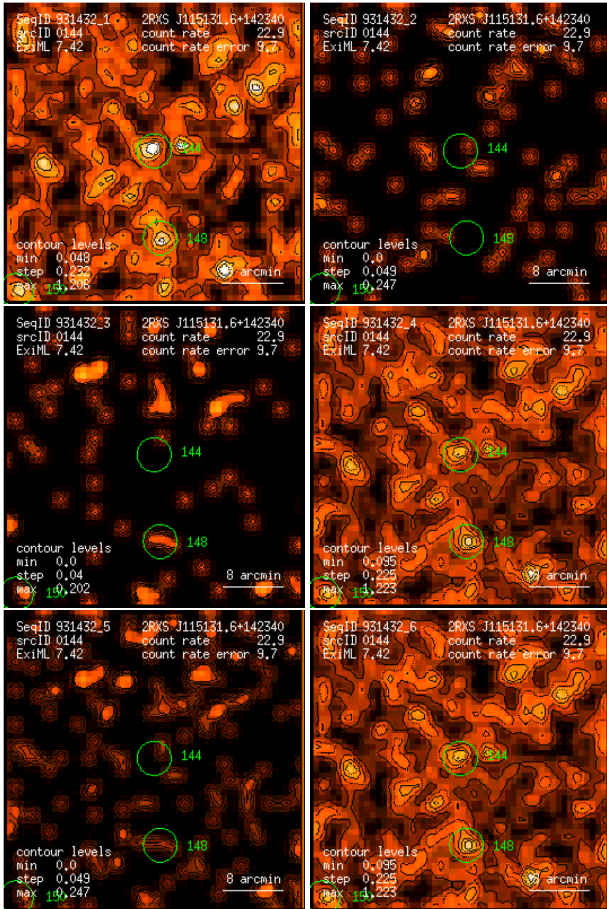
Figure 144: RASS 931432: detection 0144: band rate images, Gaussian filter: (1) PSPC channels 11 – 41, (2) 52 – 90, (3) 91 – 201, (4) 11 – 235, (5) 52 – 201, (6) 11 – 201. Broad band rates in counts/ks. Band rate contour levels in counts/ks/arcmin 2 .
