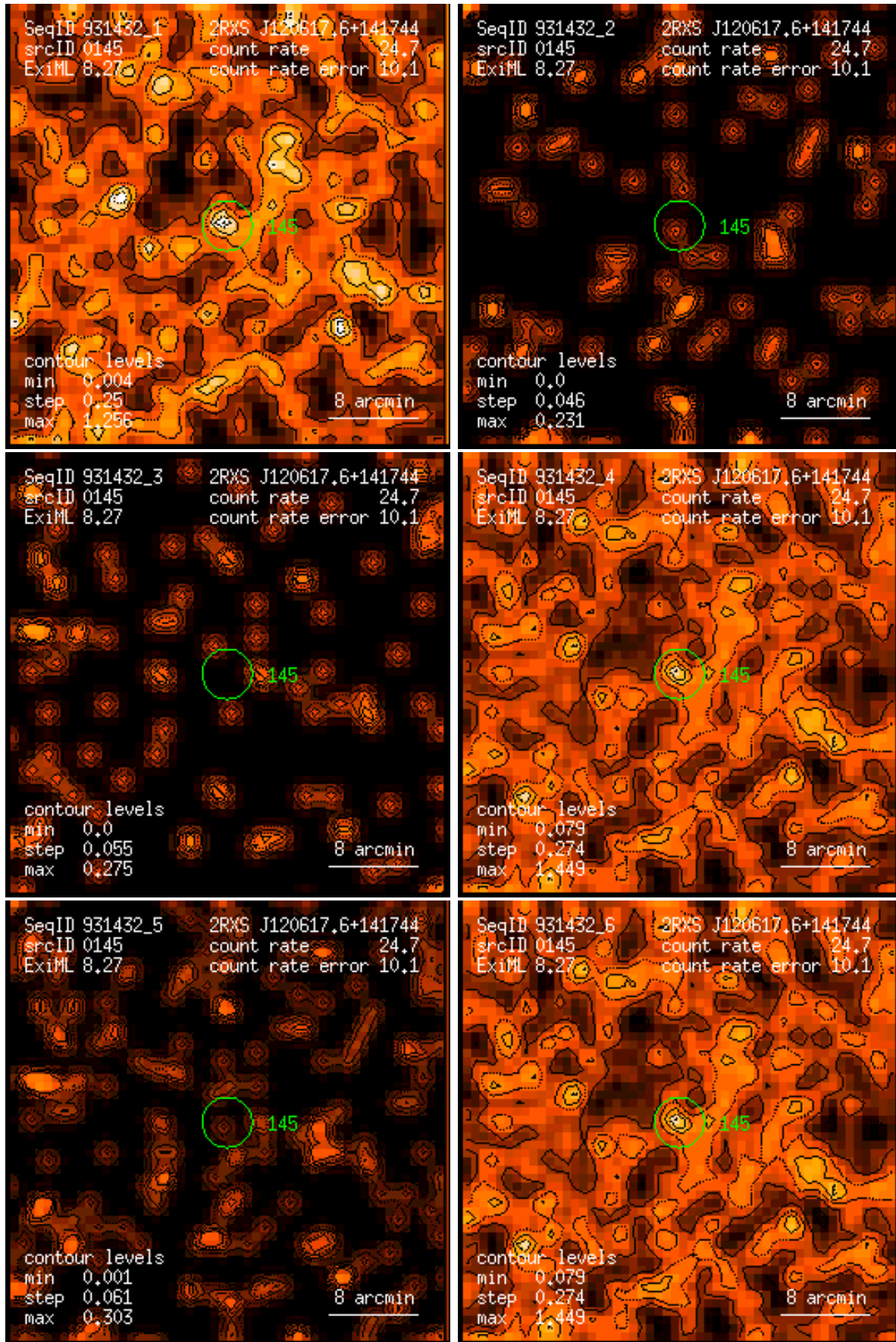
Figure 145: RASS 931432: detection 0145: band rate images, Gaussian filter: (1) PSPC channels 11 – 41, (2) 52 – 90, (3) 91 – 201, (4) 11 – 235, (5) 52 – 201, (6) 11 – 201. Broad band rates in counts/ks. Band rate contour levels in counts/ks/arcmin 2 .
