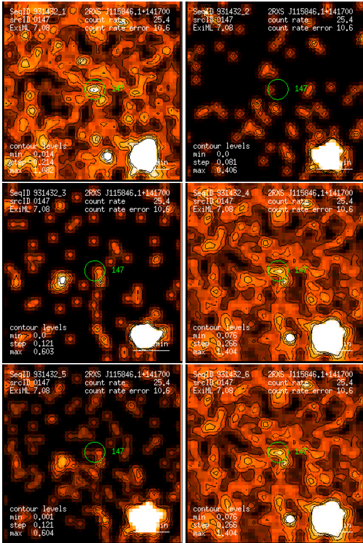
Figure 147: RASS 931432: detection 0147: band rate images, Gaussian filter: (1) PSPC channels 11 – 41, (2) 52 – 90, (3) 91 – 201, (4) 11 – 235, (5) 52 – 201, (6) 11 – 201. Broad band rates in counts/ks. Band rate contour levels in counts/ks/arcmin 2 .
