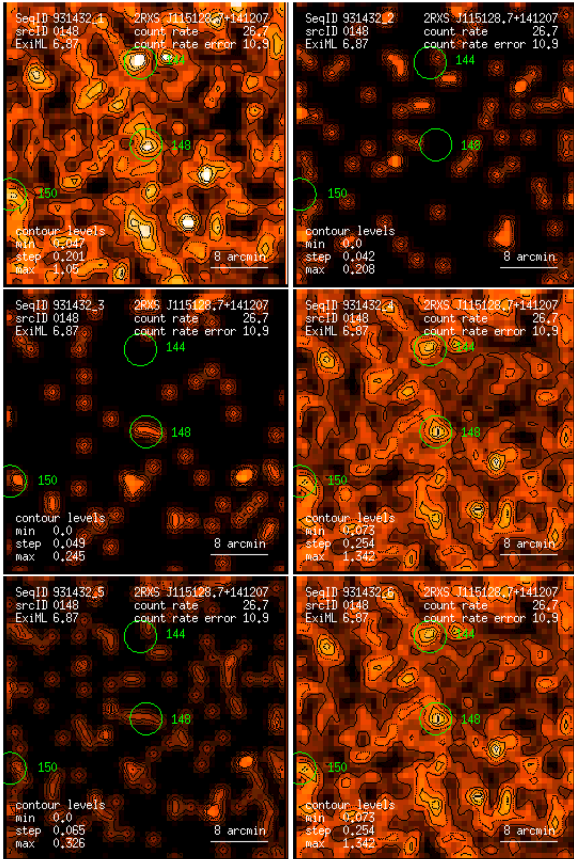
Figure 148: RASS 931432: detection 0148: band rate images, Gaussian filter: (1) PSPC channels 11 – 41, (2) 52 – 90, (3) 91 – 201, (4) 11 – 235, (5) 52 – 201, (6) 11 – 201. Broad band rates in counts/ks. Band rate contour levels in counts/ks/arcmin 2 .
